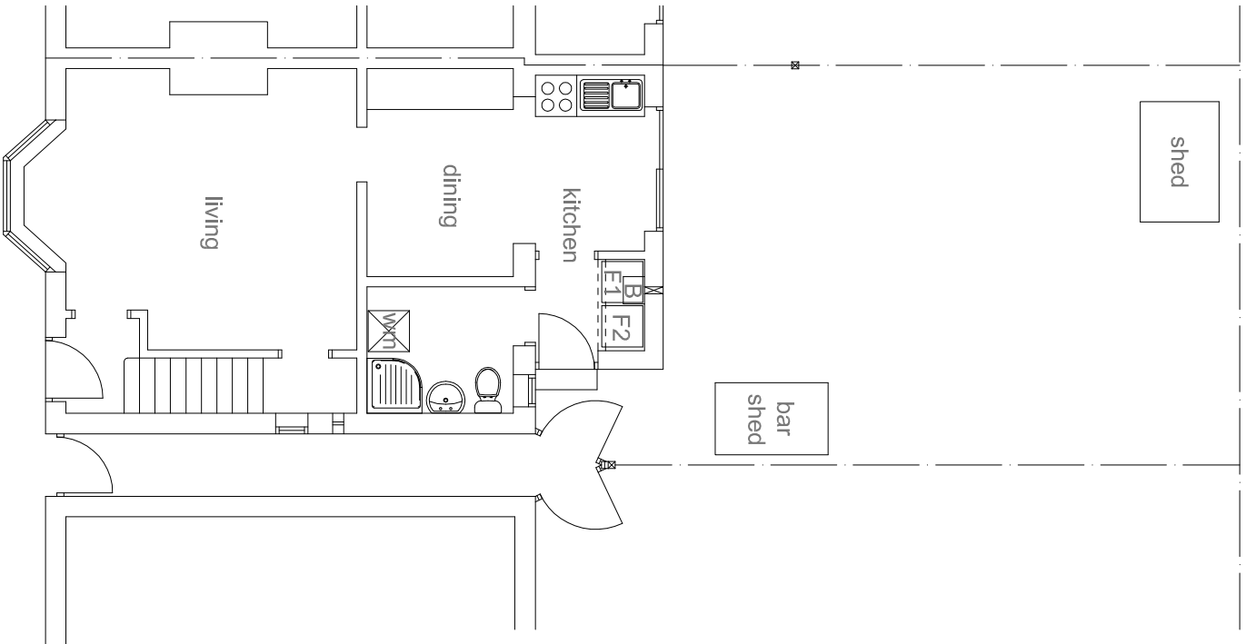
Existing ground floor plan @ 1:100 scale
