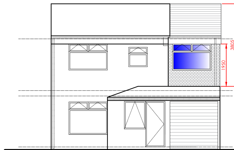
Proposed Principle Elevation Scale - 1:100
