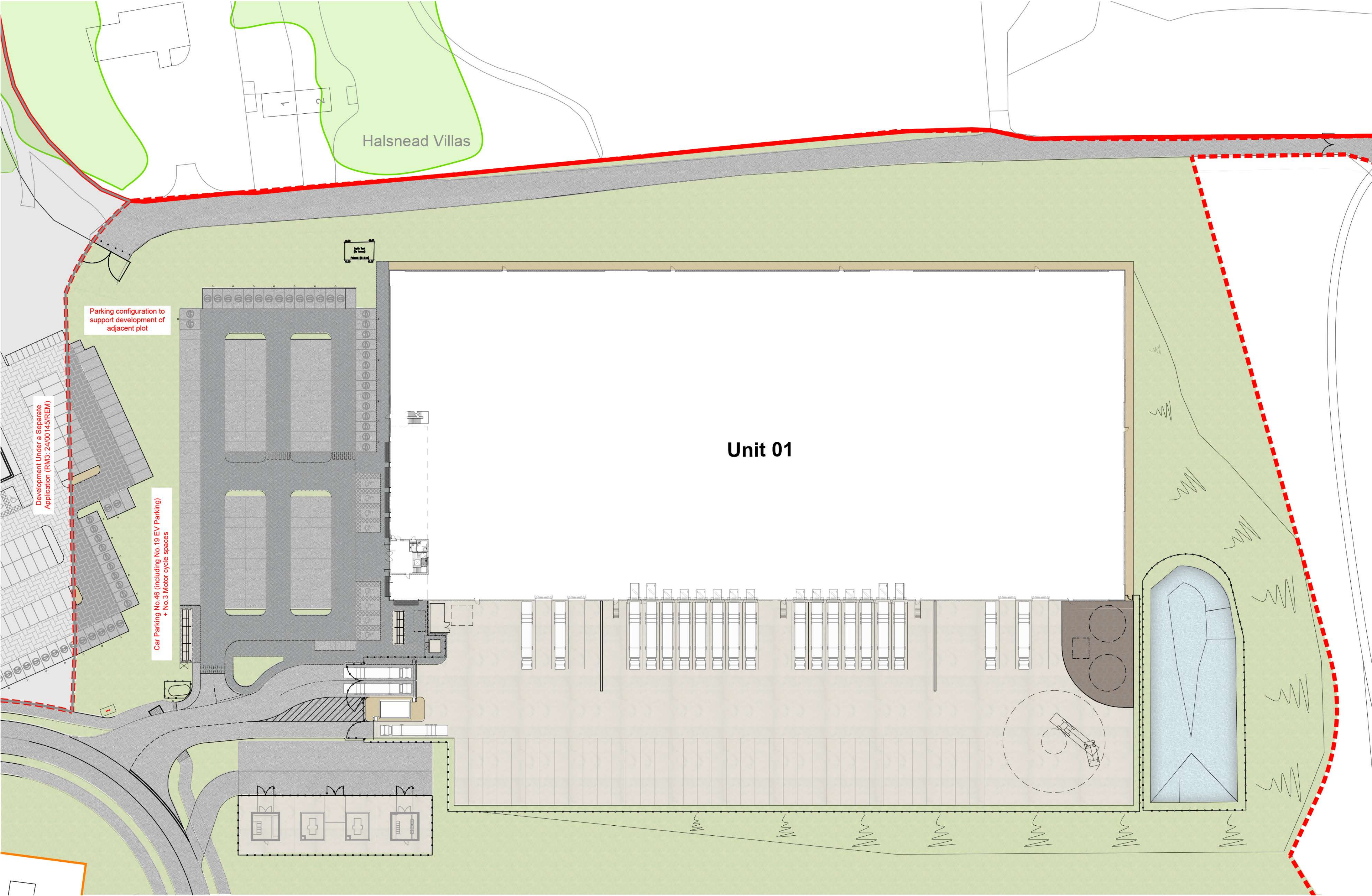
Unit 01 External Finishes Plan Scale 1:500
