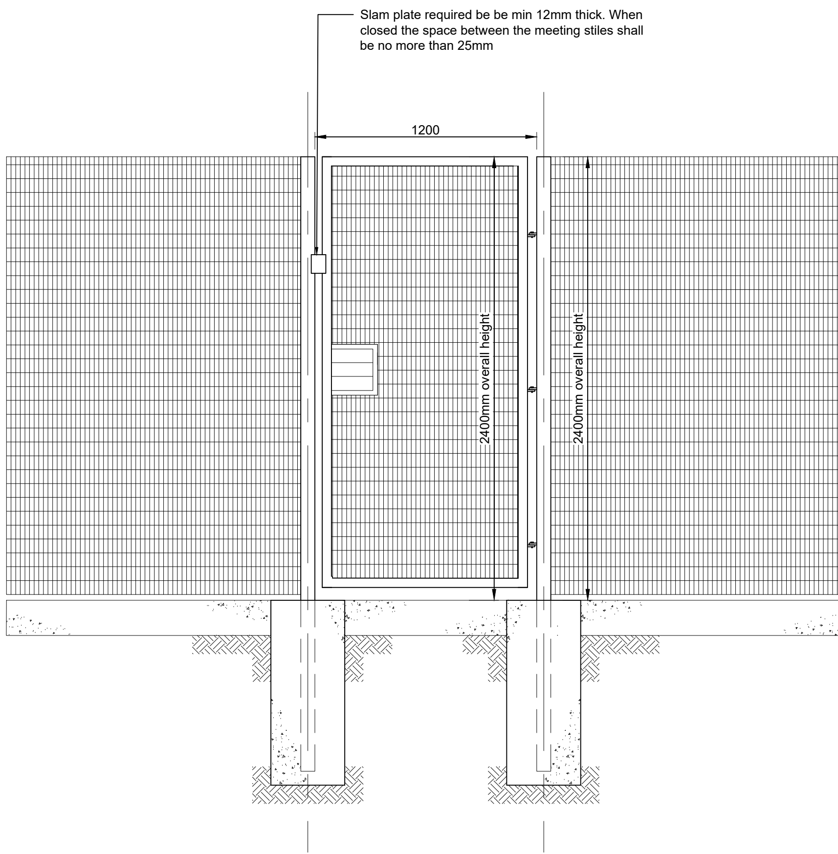
Personnel Gate Details Scale 1:20
