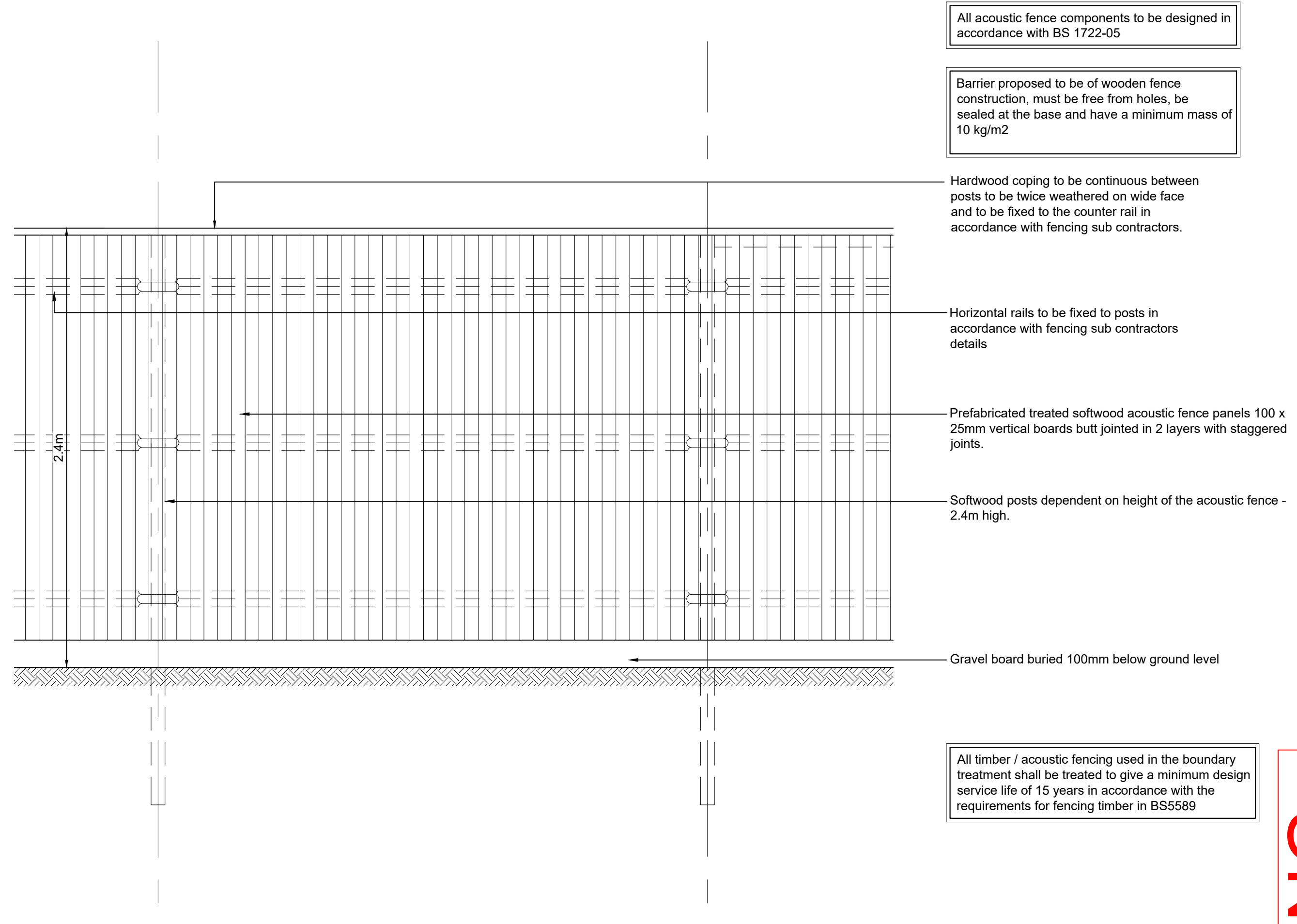
Acoustic Fencing Scale 1:20
