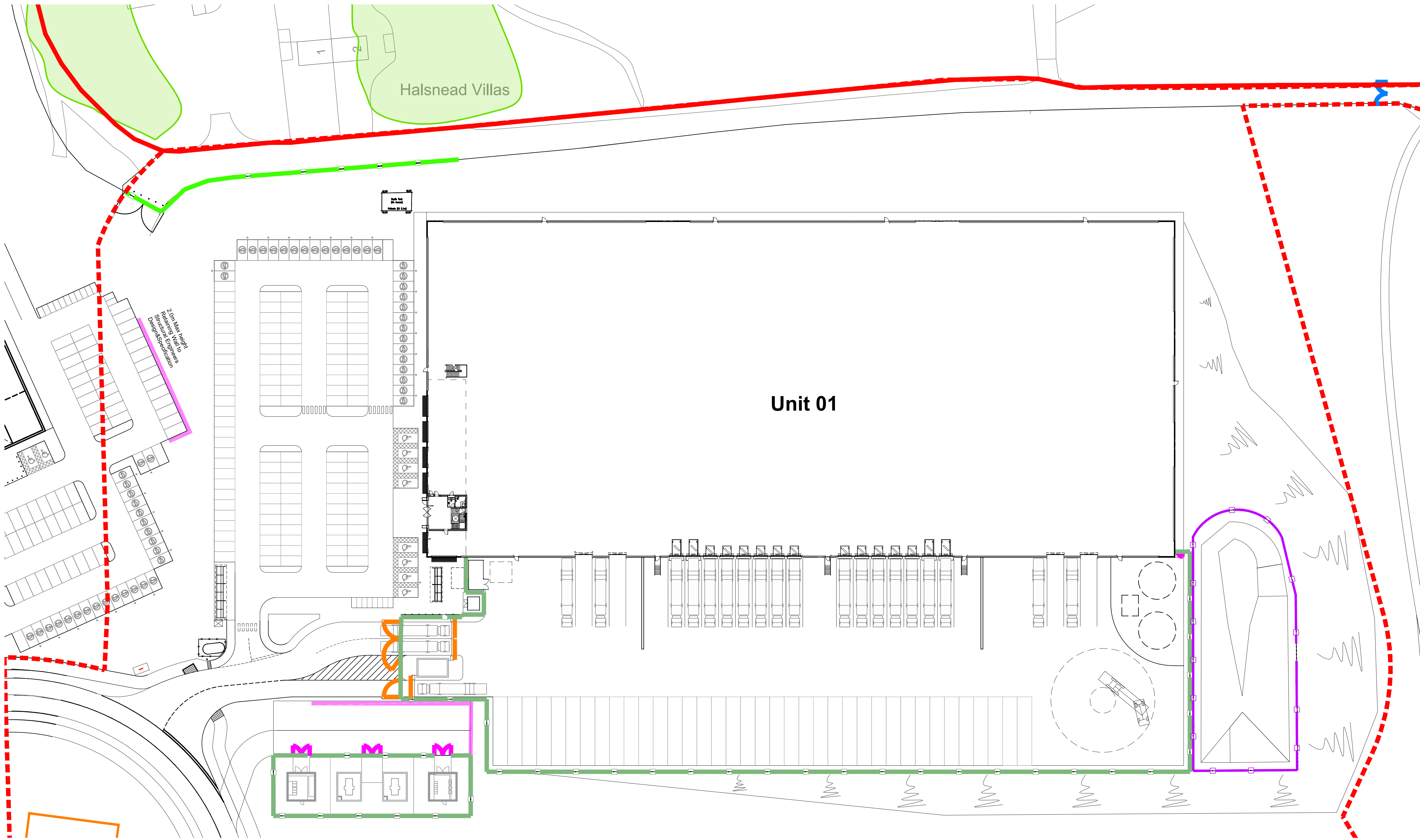
Fencing Plan Scale 1:500
