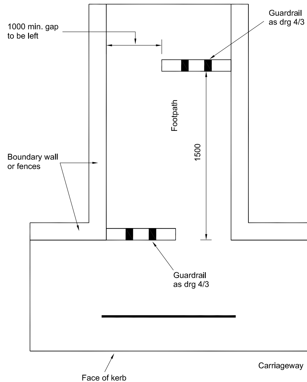
Alternative layouts for Pedestrian Guardrails at end of Footpaths
