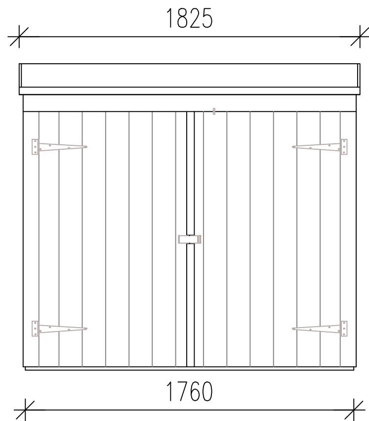
FRONT ELEVATION
