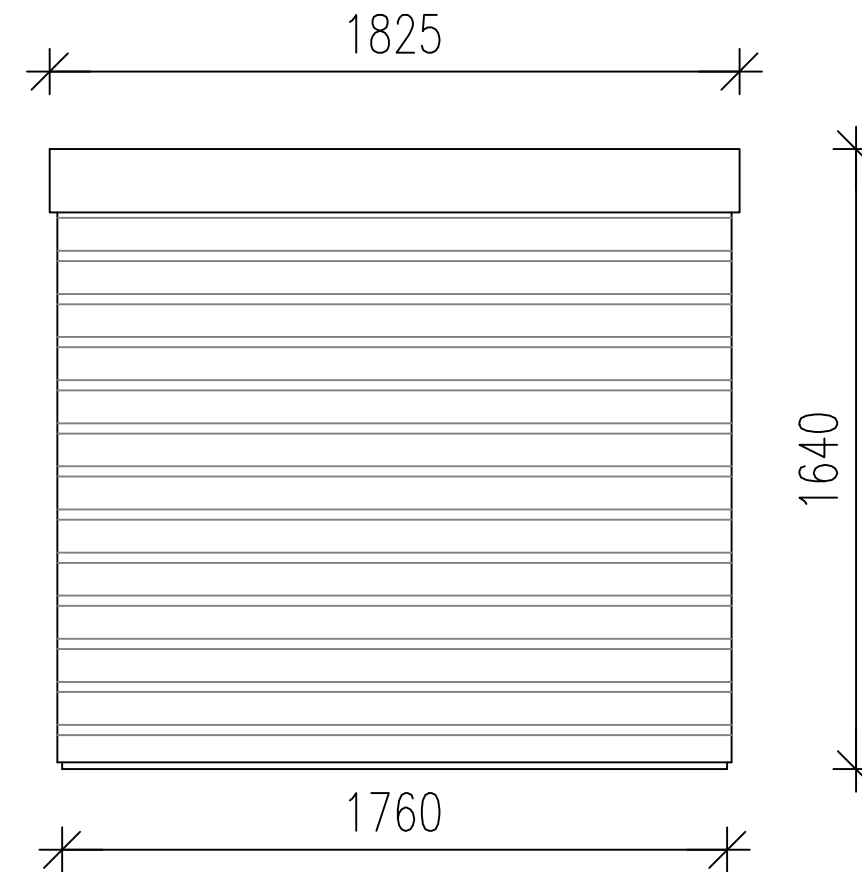
REAR ELEVATION
