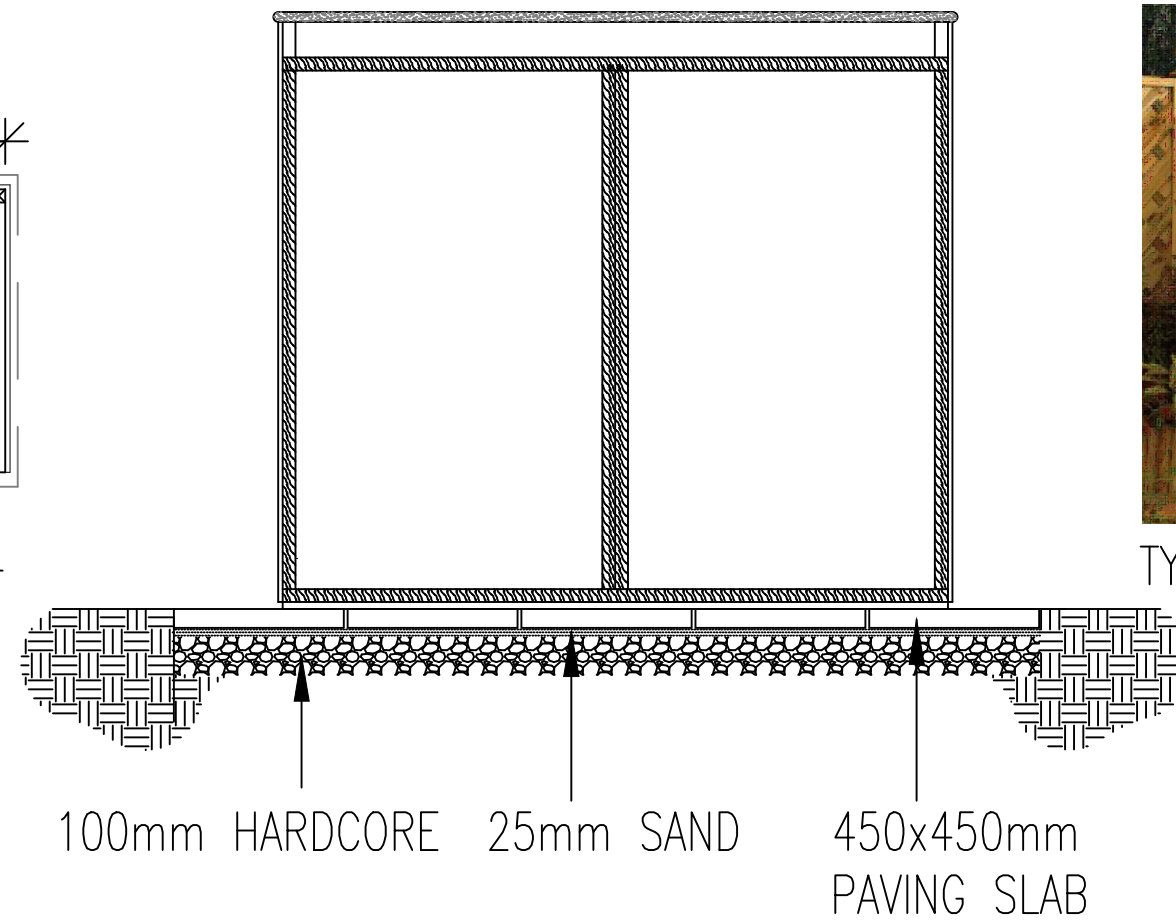
TYPICAL SECTION
