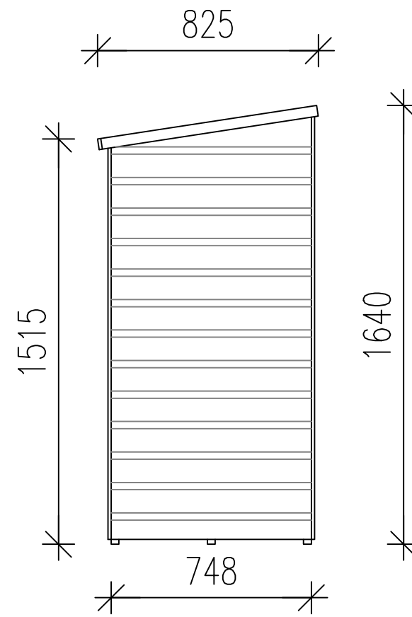
SIDE ELEVATION
