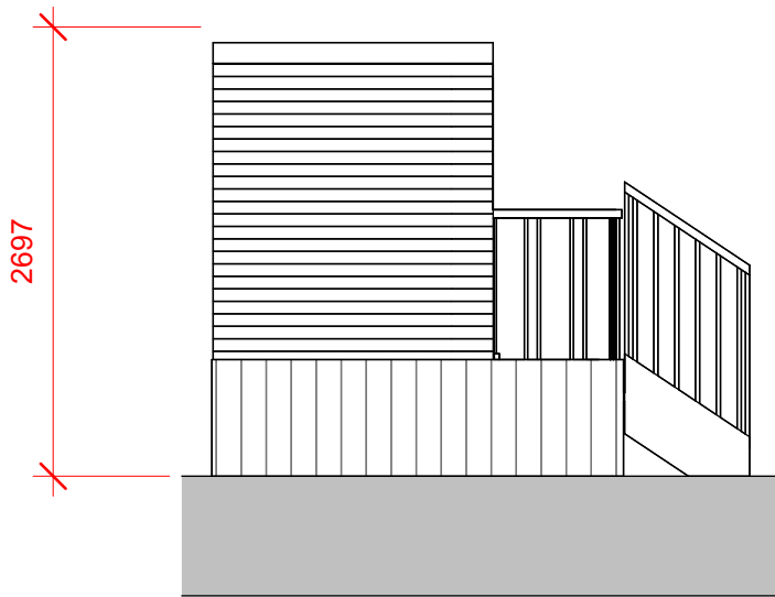
OB 2 East Elevation 1 : 50
