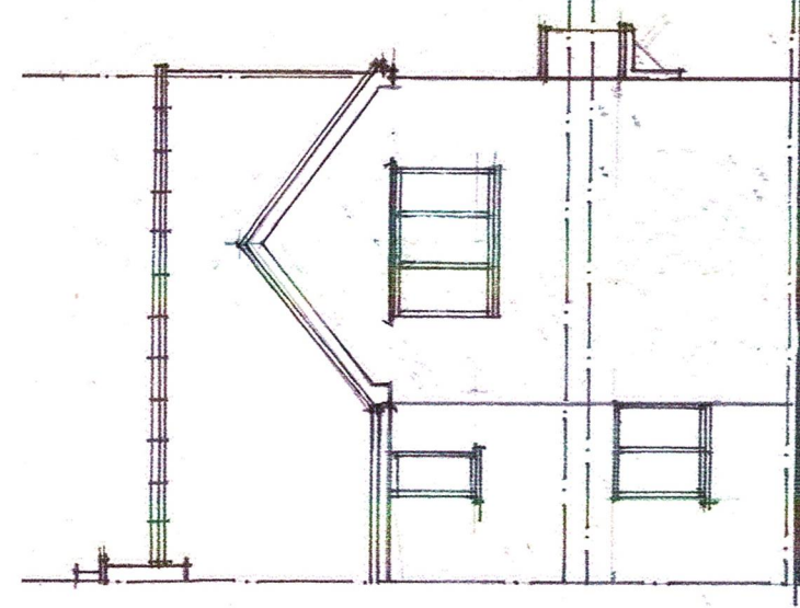
Rear Elevation as proposed scale 1:100 @ A3
