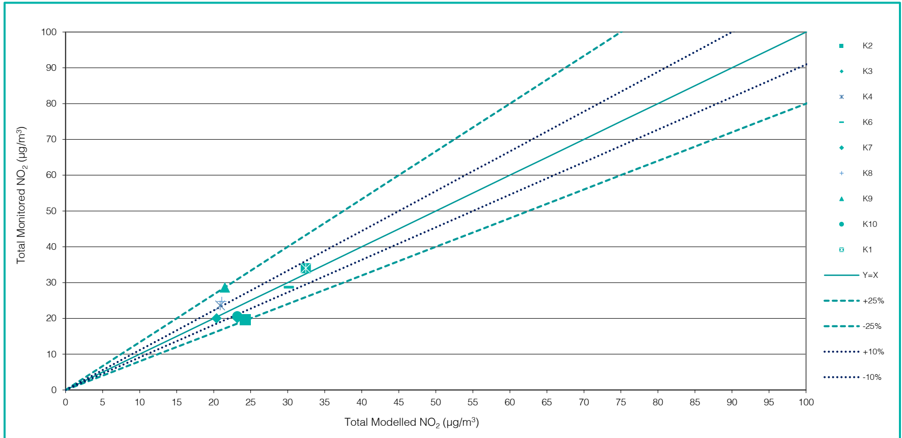
Figure 7.5.2: Comparison of Monitored and Modelled NO 2 Concentrations After Adjustment
