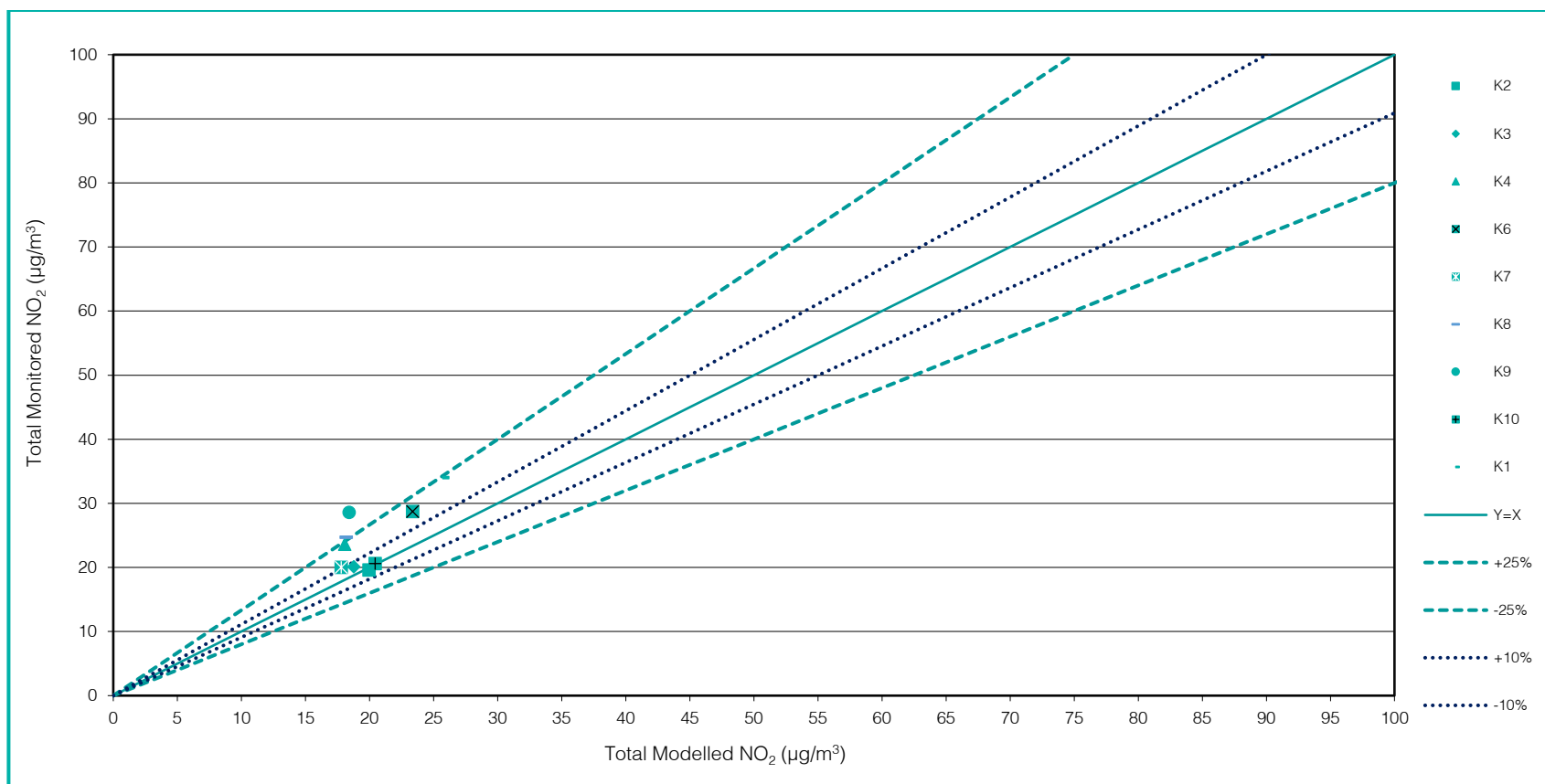
Figure 7.5.1: Comparison of Monitored and Modelled NO 2 Concentrations Before Adjustment
