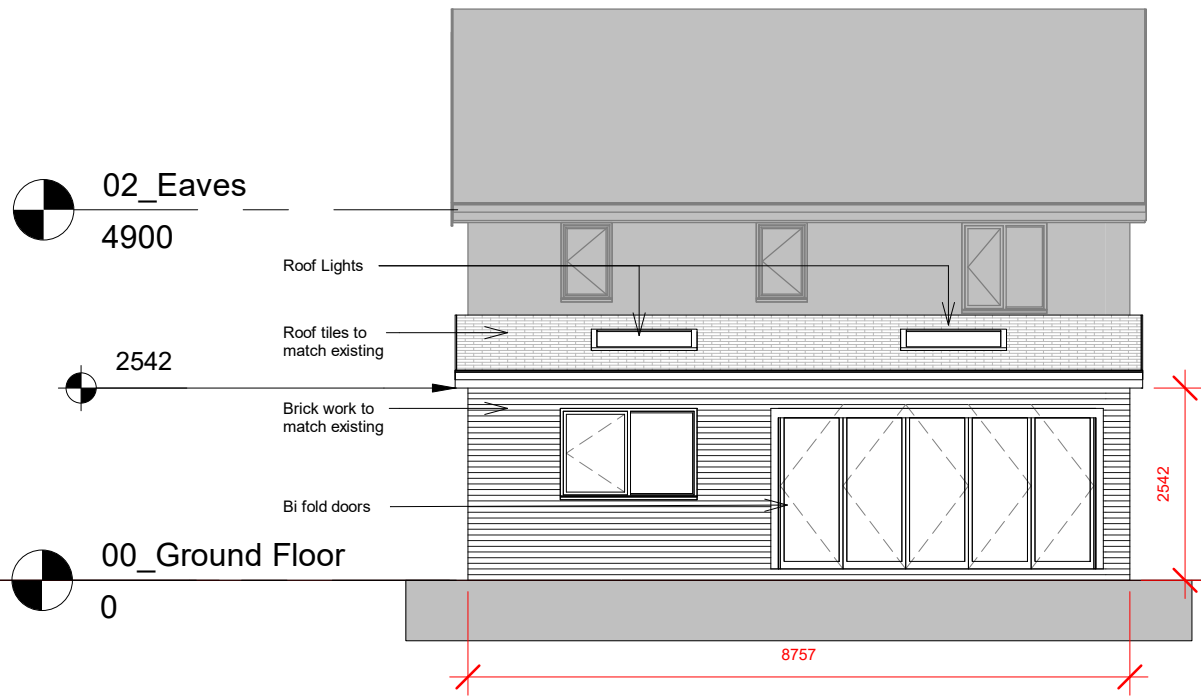
Rear Elevation 1 : 100
