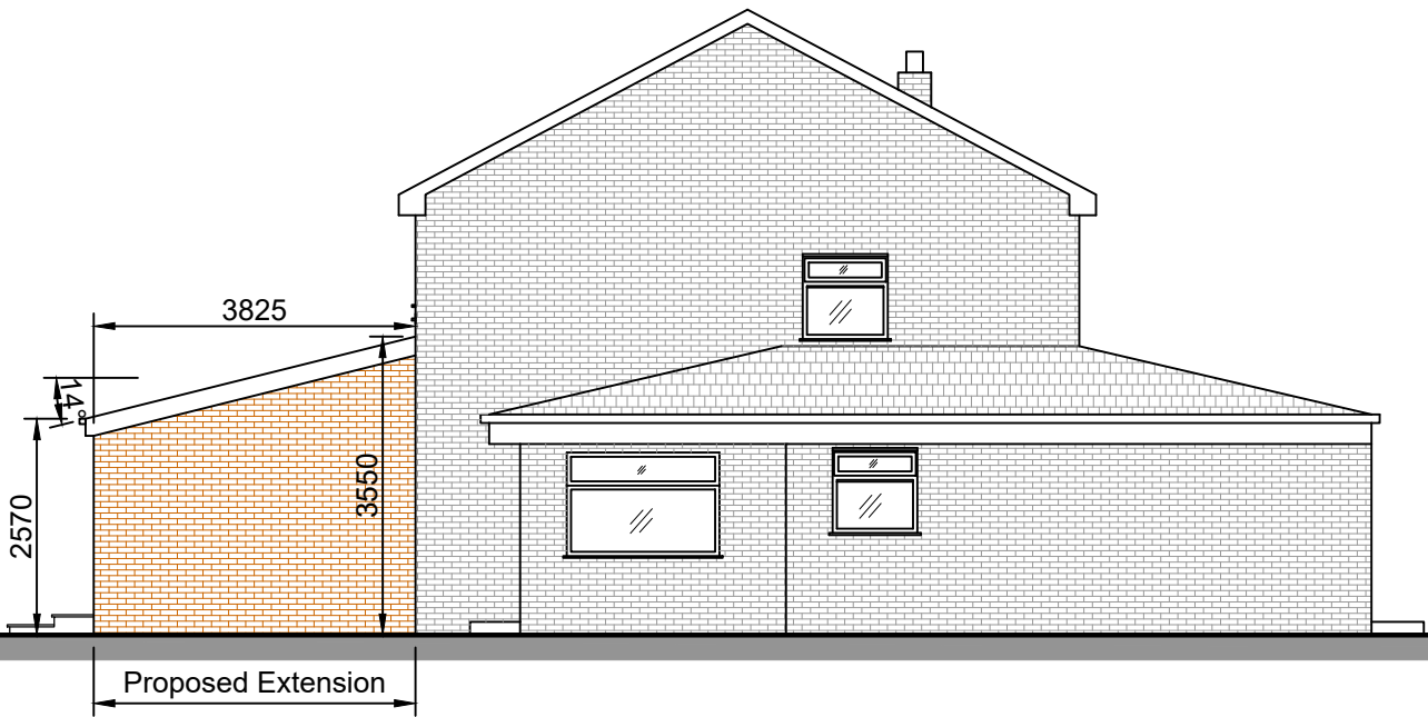
Proposed Side Elevation. North West.
