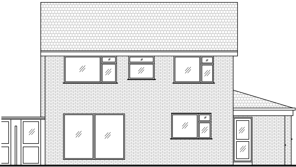
Existing Rear Elevation. North East.
