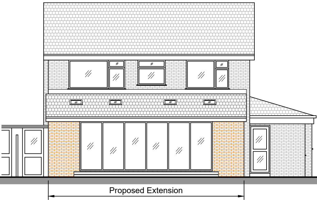
Proposed Rear Elevation. North East.
