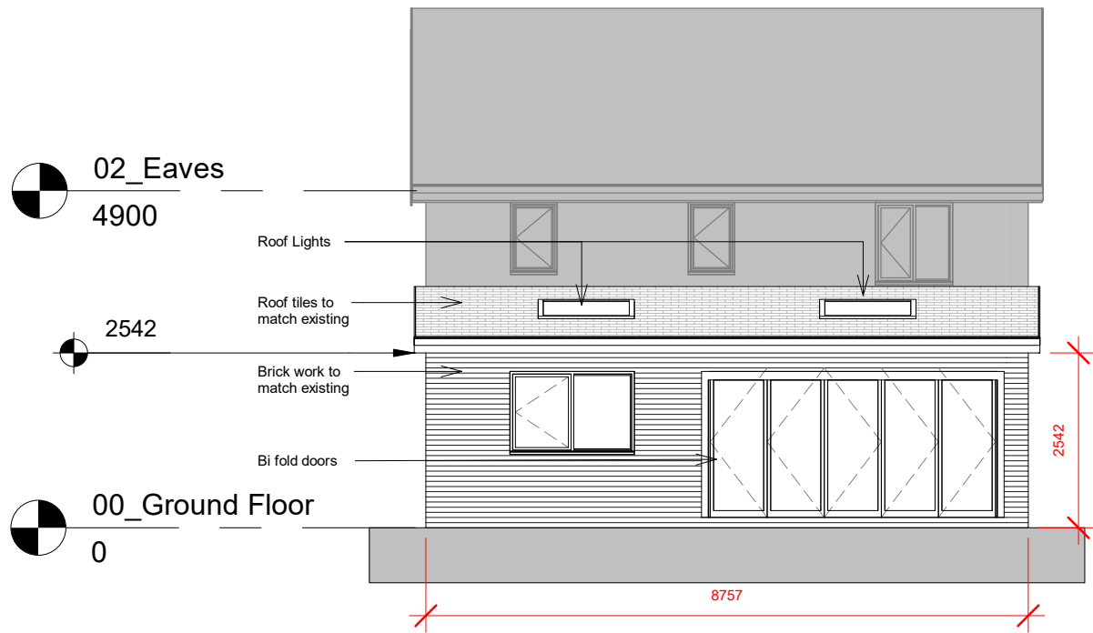
Rear Elevation
