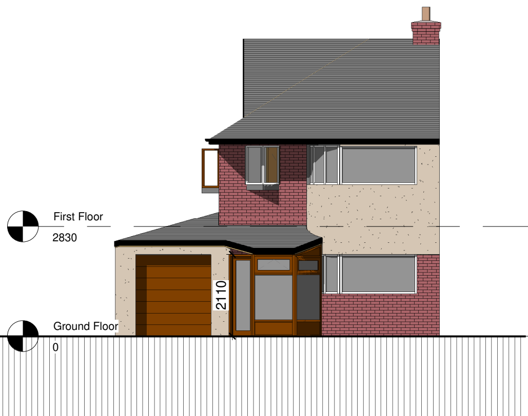
Front Elevation 1 : 100
