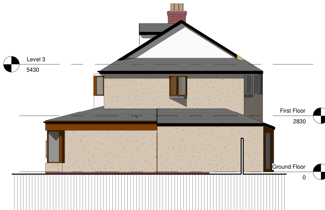
Side Elevation 1 : 100
