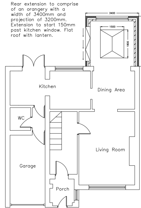
Proposed Ground Floor
