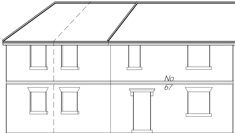
SOUTH WEST
