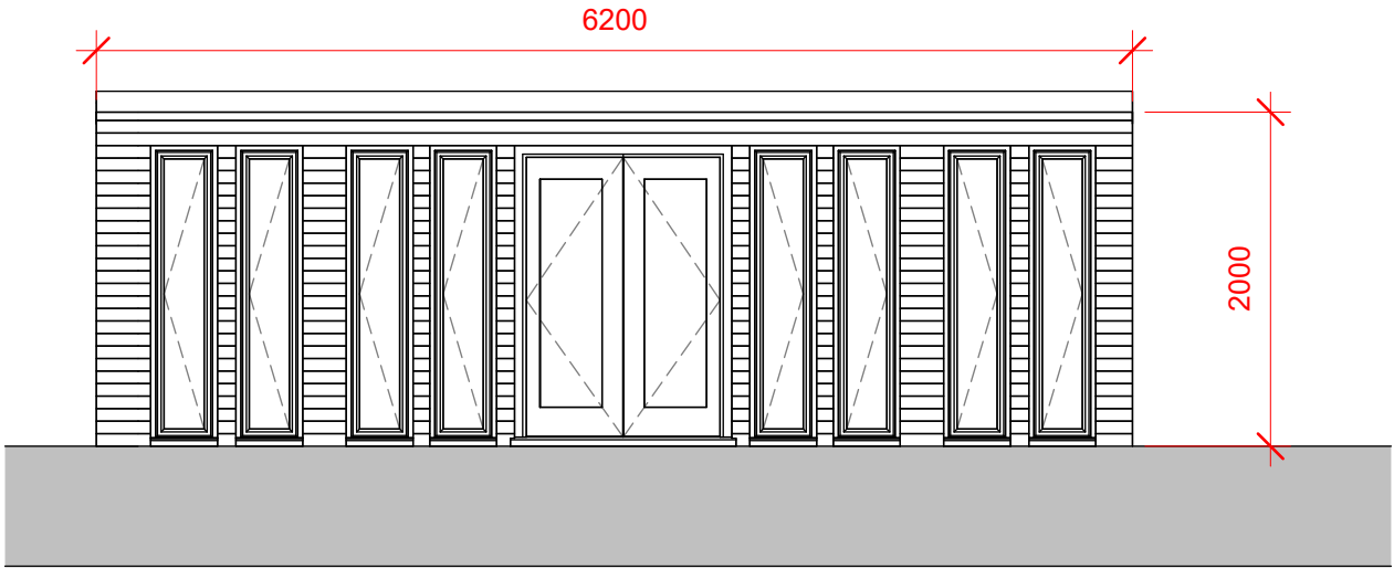
OB 1 Front Elevation 1 : 50
