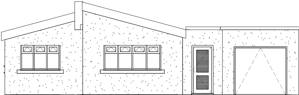
Front Elevation 1 : 100
