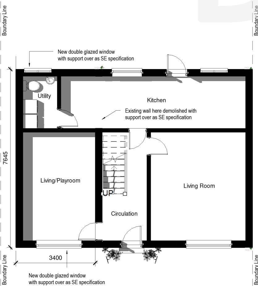
1 Level 0 - Proposed 1 : 100
