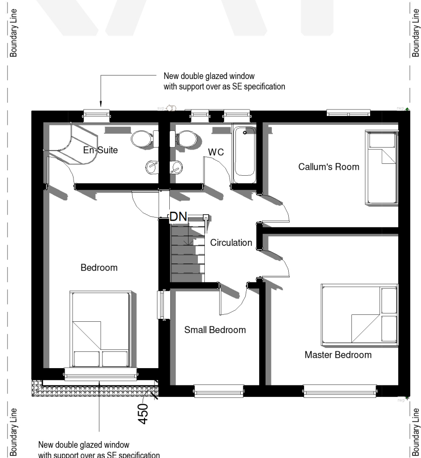
2 Level 01 - Proposed 1 : 100
