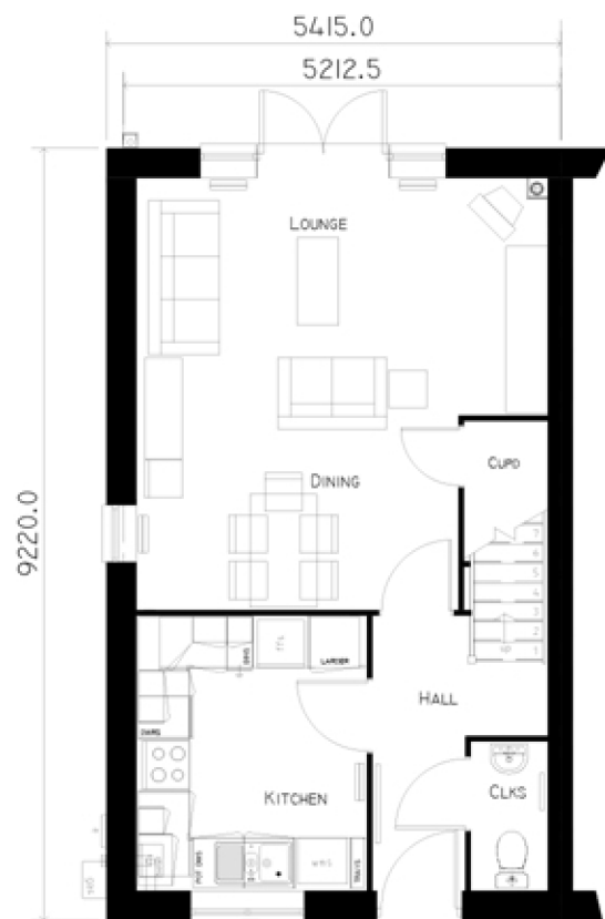
GROUND FLOOR PLAN GFA 41.83M2 (41.03M2)
