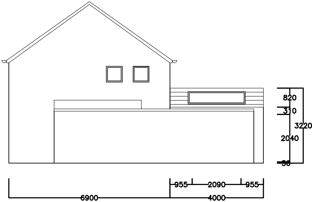
Proposed Right Hand Elevation
