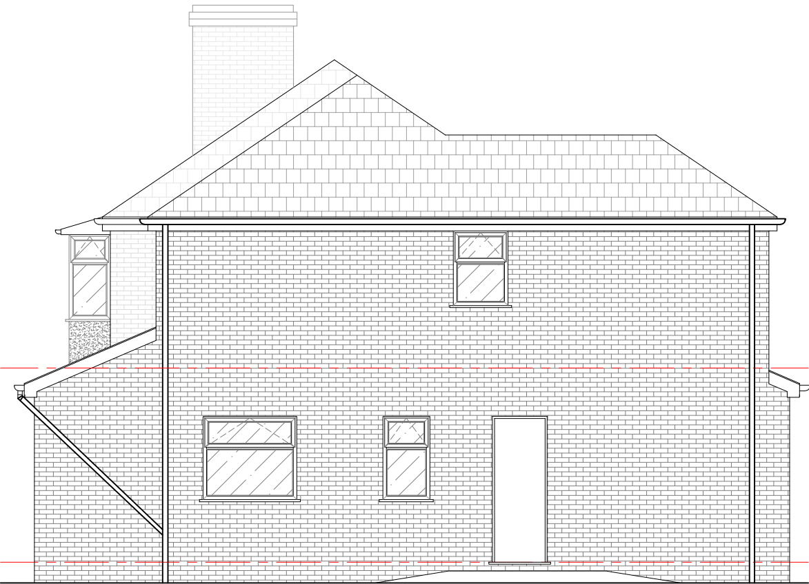
Proposed Side Elevation (Scale - 1:75)
