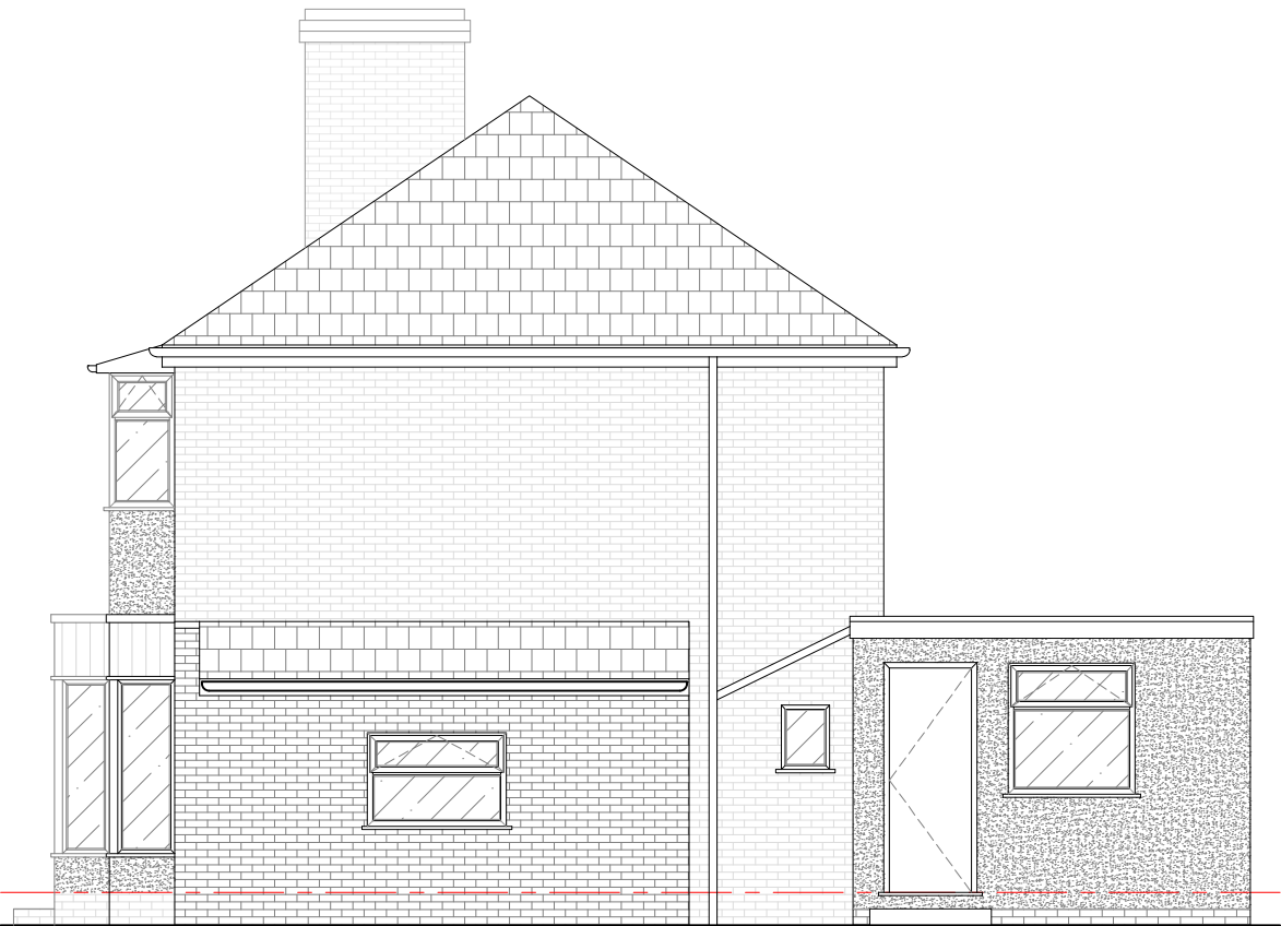
Existing Side Elevation (Scale - 1:75)
