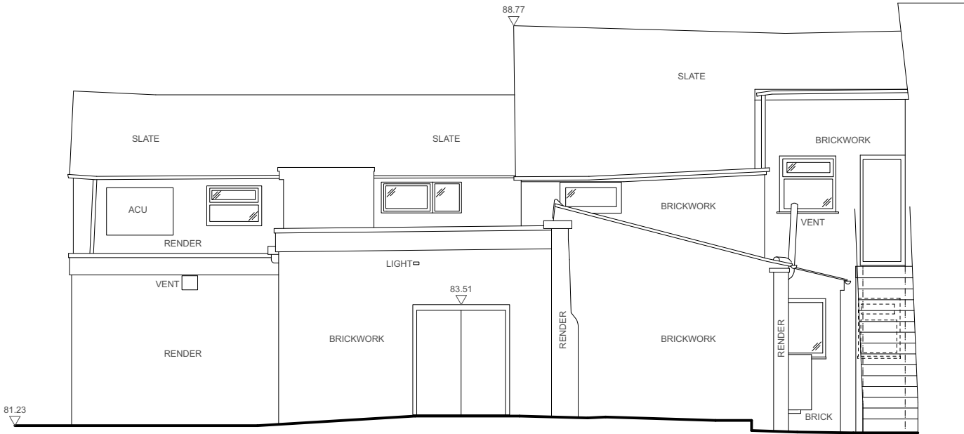
Existing Elevation: North
