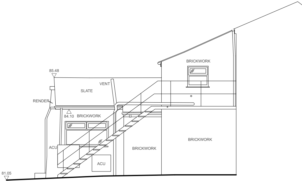
Existing Elevation: West
