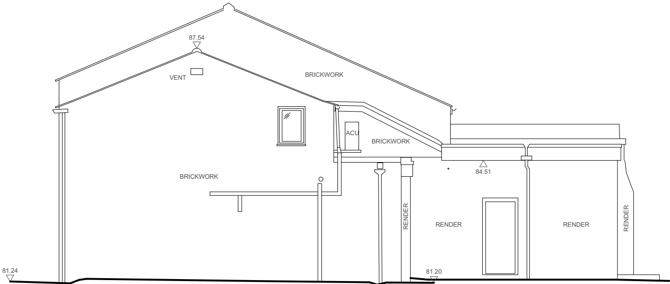
Existing Elevation: East
