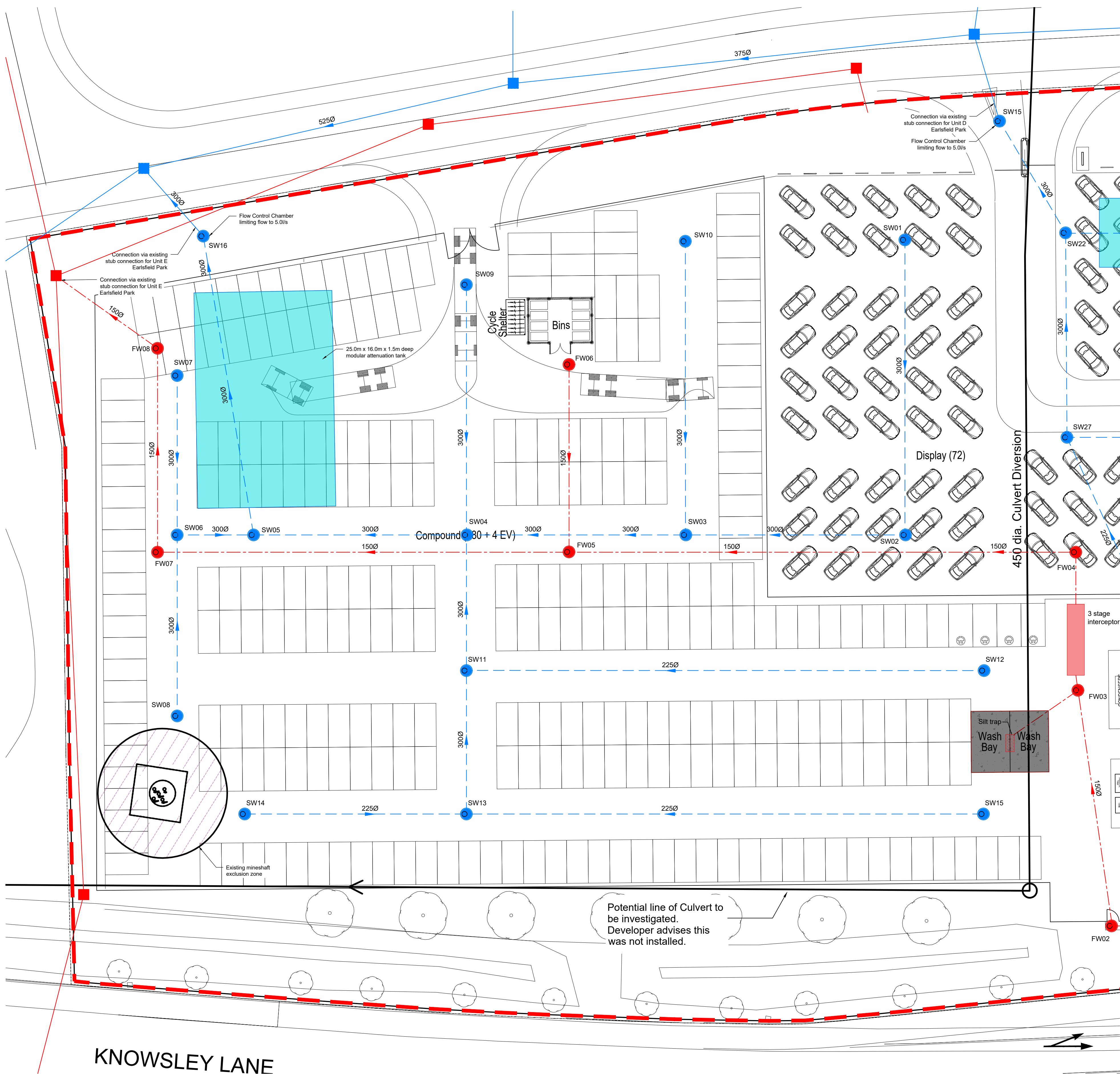
DRAINAGE STRATEGY VIEW 1 Scale: 1:250
