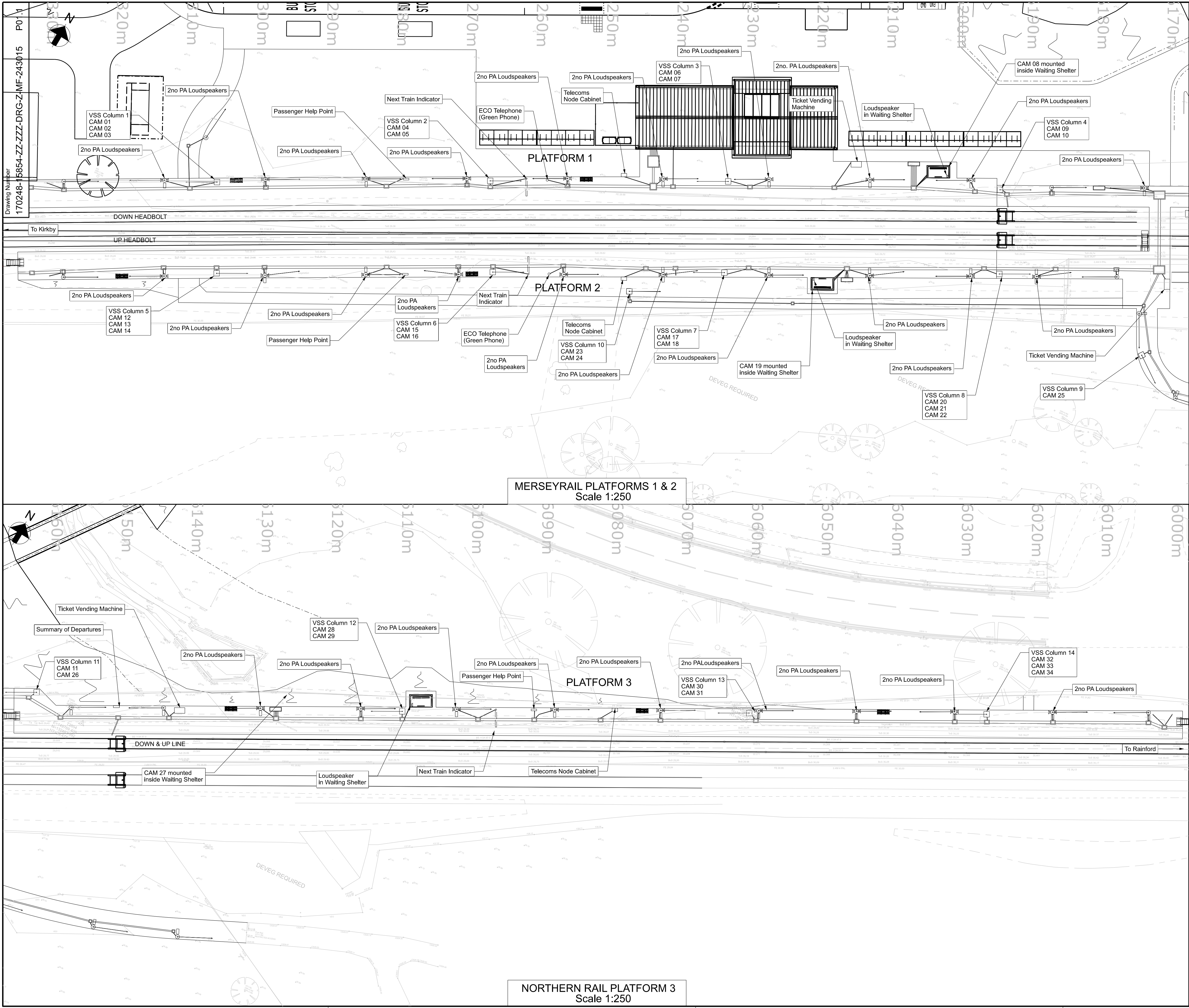
Figure 2.17b: Station Platform Tannoy and Telecommunications GA
