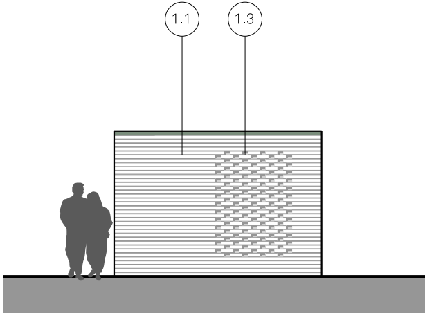
SOUTH ELEVATION
