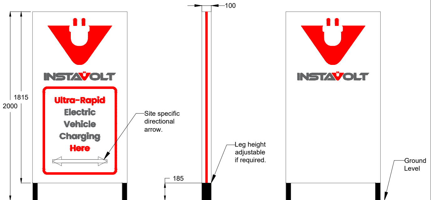
A Totem - Front View
