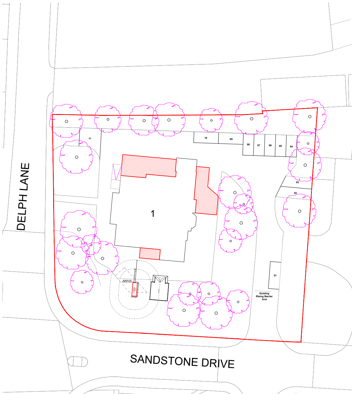
10m 0 10m SITE PLAN @ 1:500
