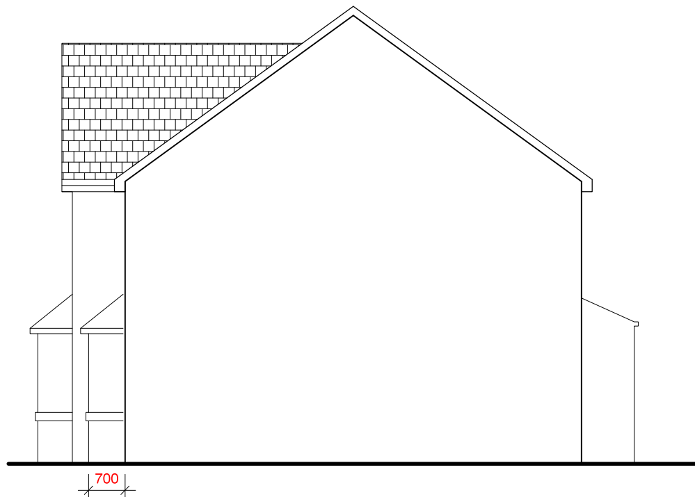
SIDE ELEVATION - WEST PROPOSED
