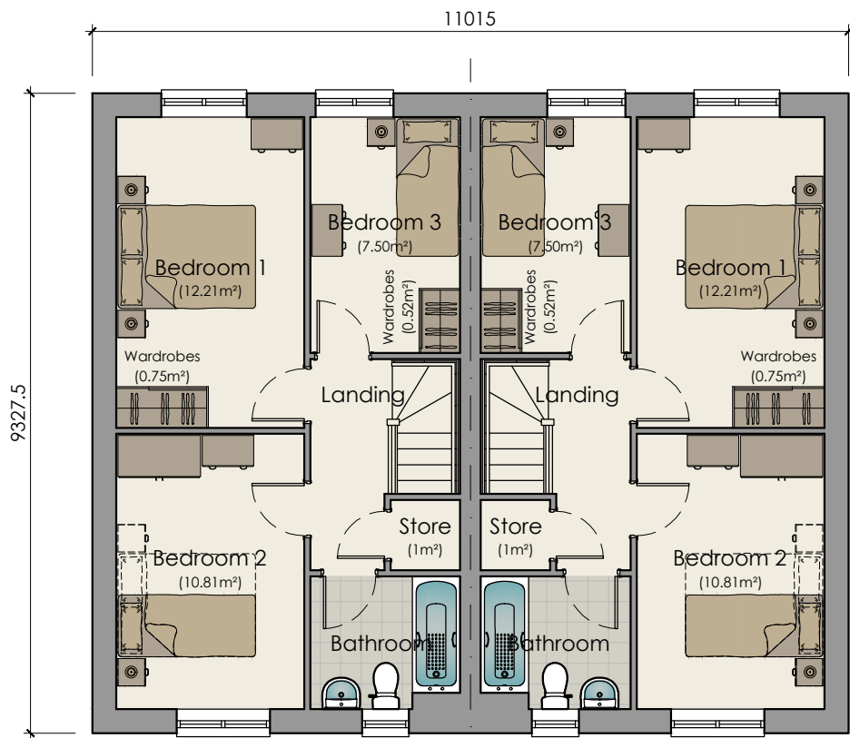
TYPE F - LtF 3B4P 86 (AS) FIRST FLOOR PLAN - Semi-Detached
