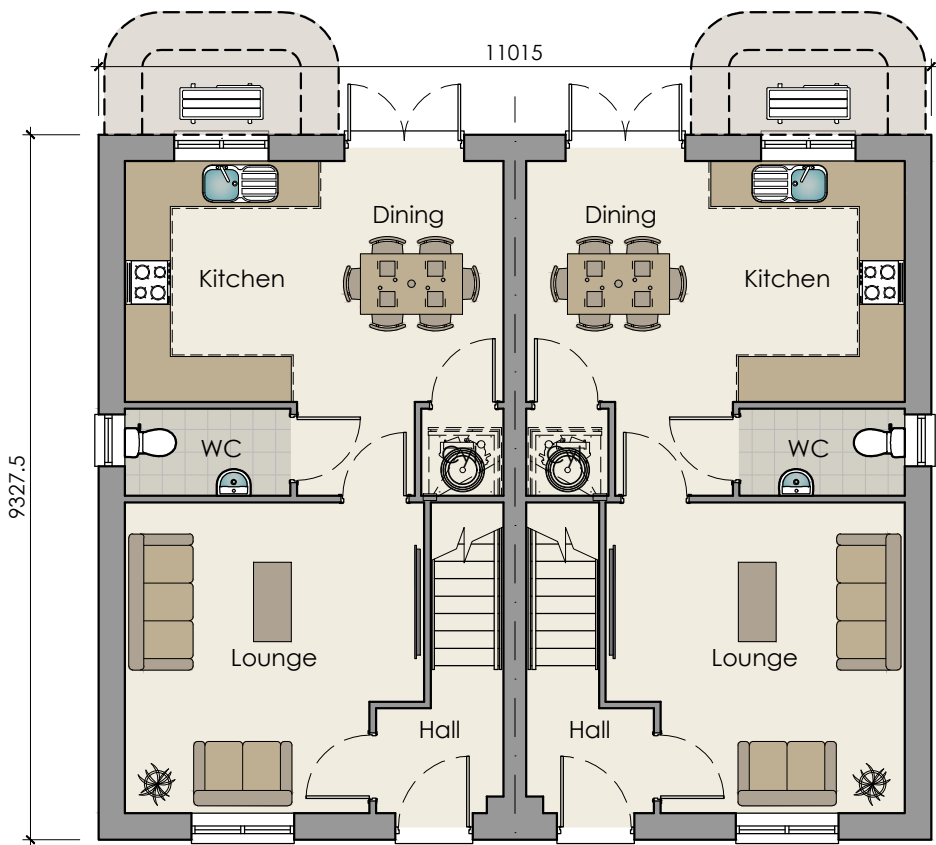
TYPE F - LtF 3B4P 86 (AS) GROUND FLOOR PLAN - Semi-Detached
