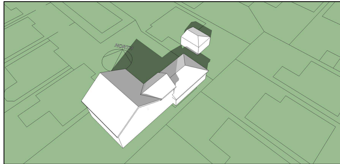
Proposed - 12pm Winter Solstice
