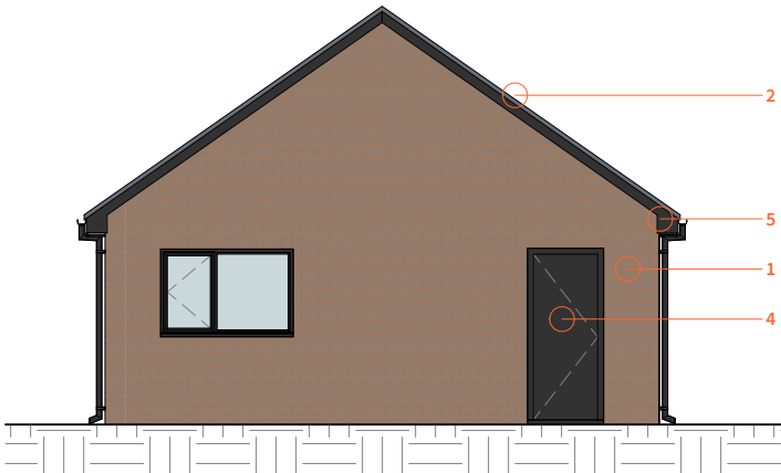
LHS Elevation
