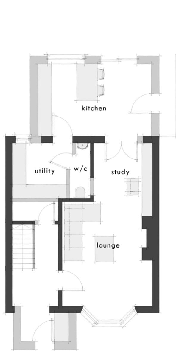
proposed ground floor plan scale 1:100
