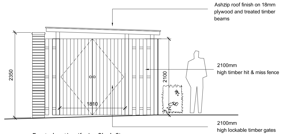
Front elevation (facing Block C)
