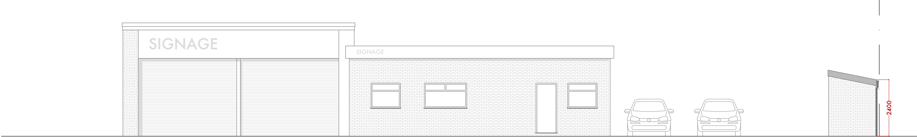
01 Front Elevation (1:100)
