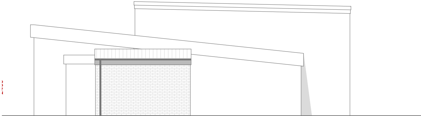
03 Side Elevation (1:100)
