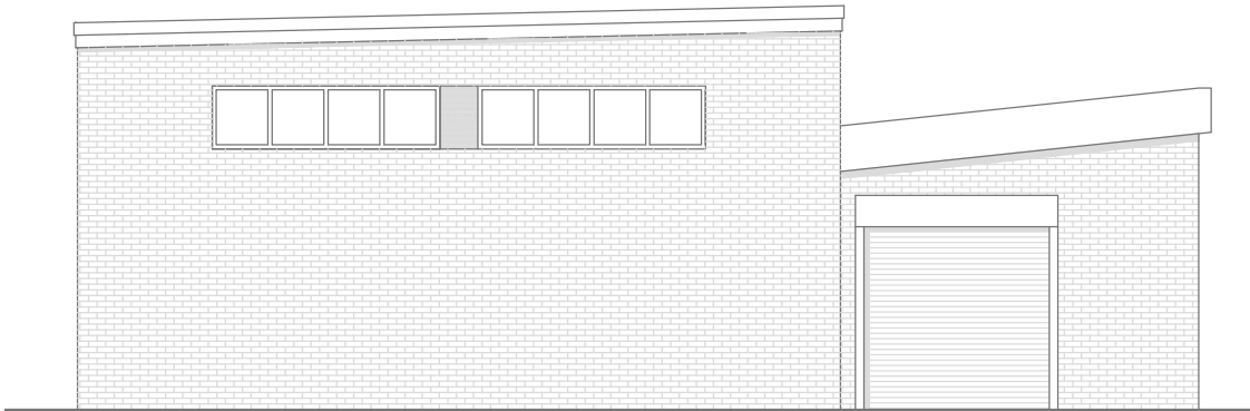
02 Side Elevation (1:100)
