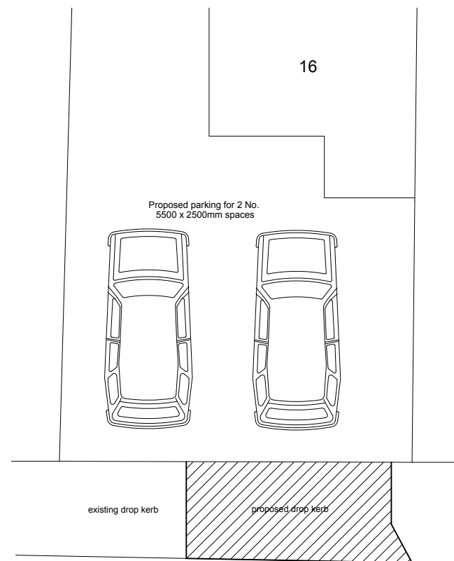
Proposed Plan
