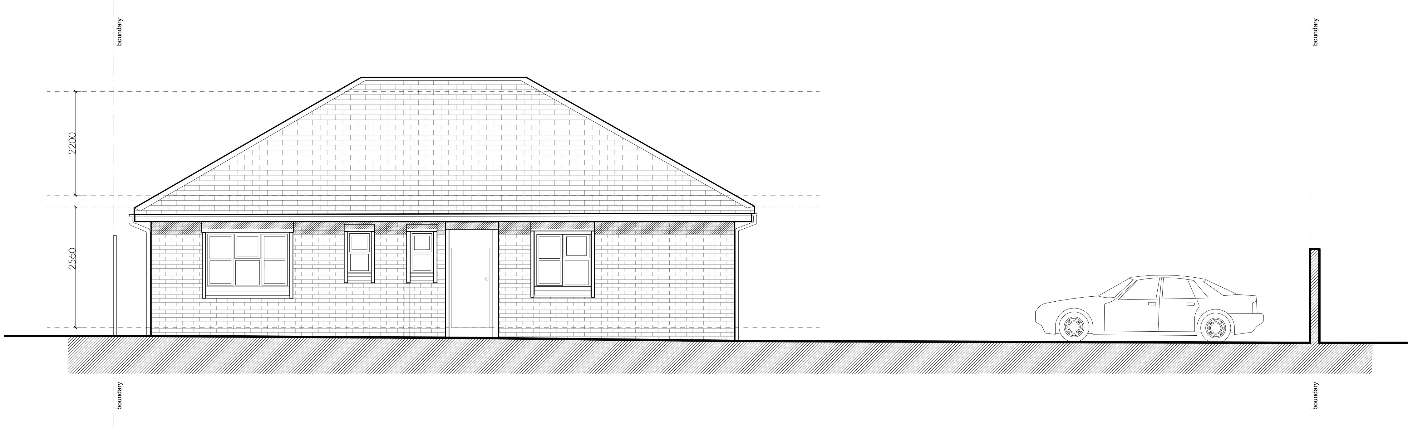
PROPOSED REAR ELEVATION 1:50 Scale
