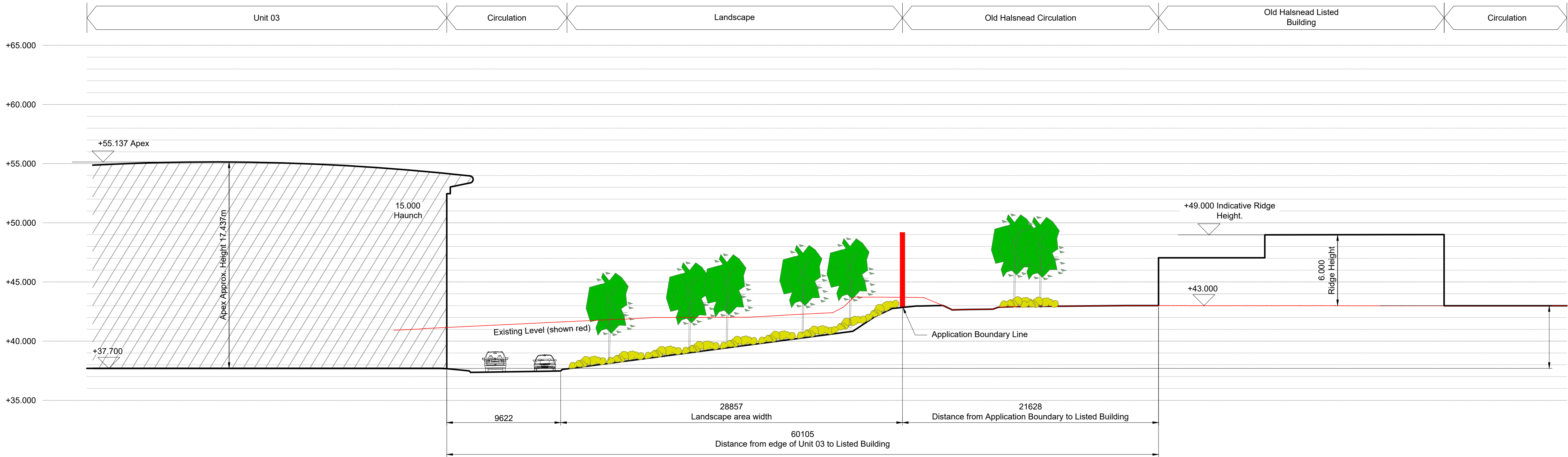
Unit 03 Site Cross Section (A-A) Scale 1:200
