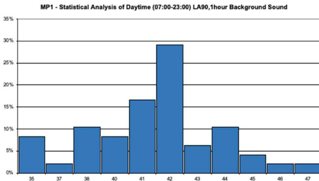
FIGURE 8: STATISTICAL ANALYSIS OF LA90 BACKGROUND – DAYTIME – MP1
