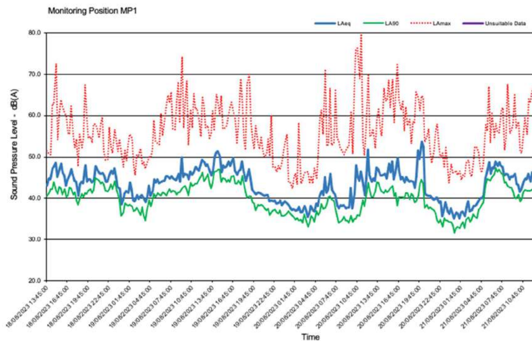
FIGURE 6: MEASURED TIME HISTORY – MP1
