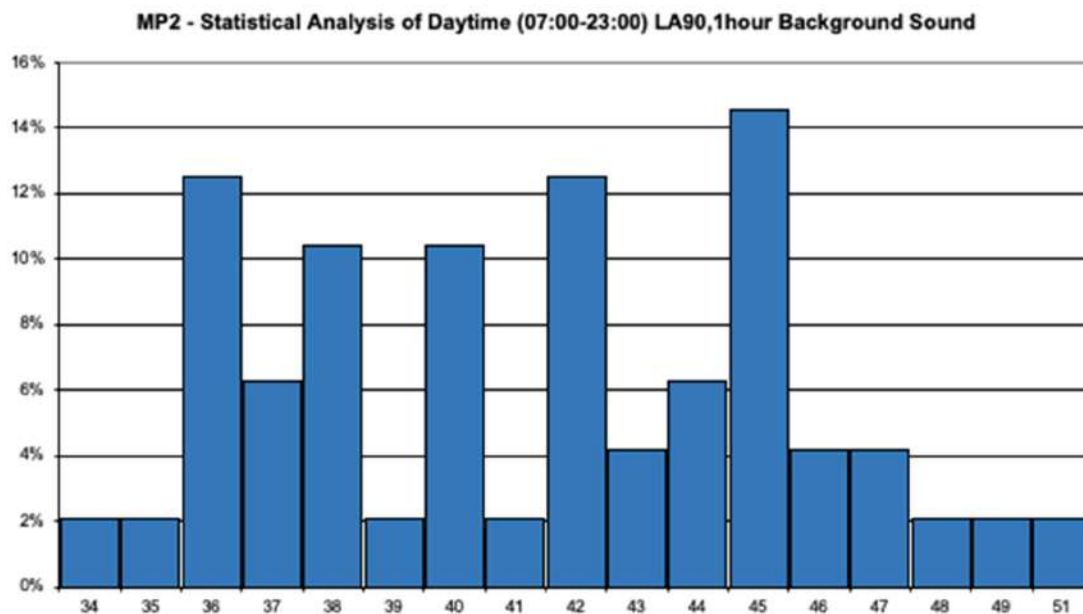
FIGURE 10: STATISTICAL ANALYSIS OF LA 90 BACKGROUND – DAYTIME – MP2
