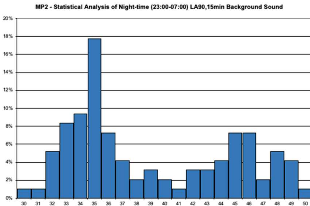
FIGURE 11: STATISTICAL ANALYSIS OF LA 90 BACKGROUND – NIGHT-TIME – MP2
