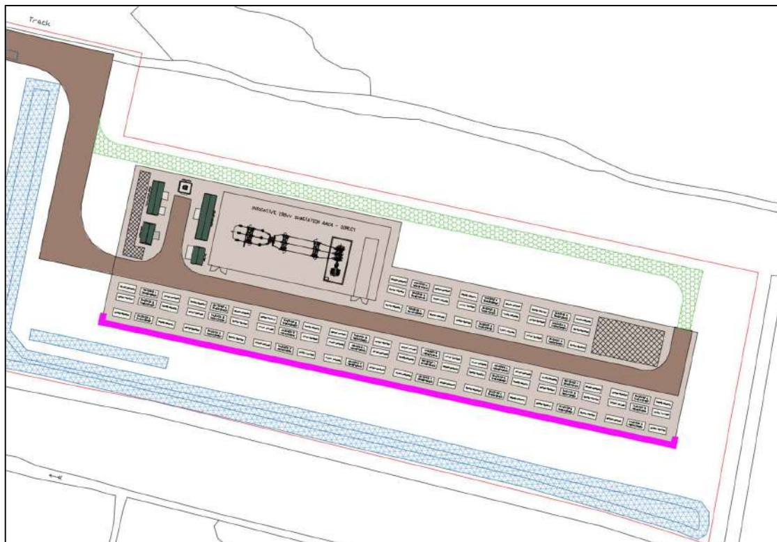
FIGURE 4: PROPOSED 4.5M HIGH NOISE FENCE
