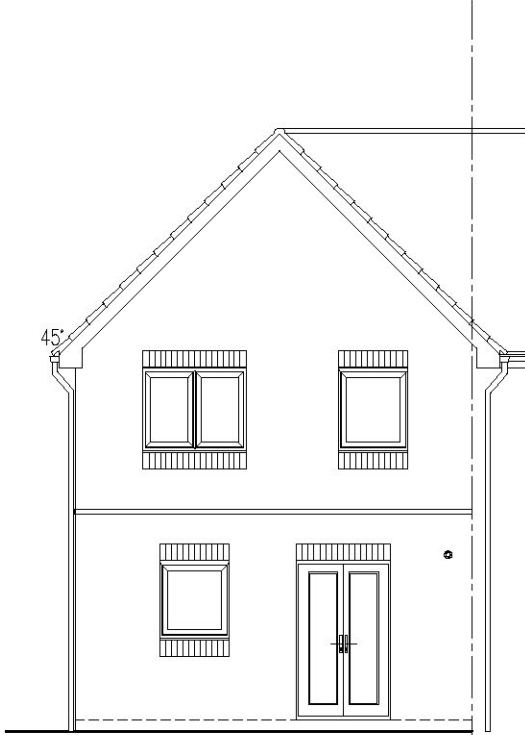
REAR ELEVATION END/SEMI DETACHED EMA32 (3B5P)
