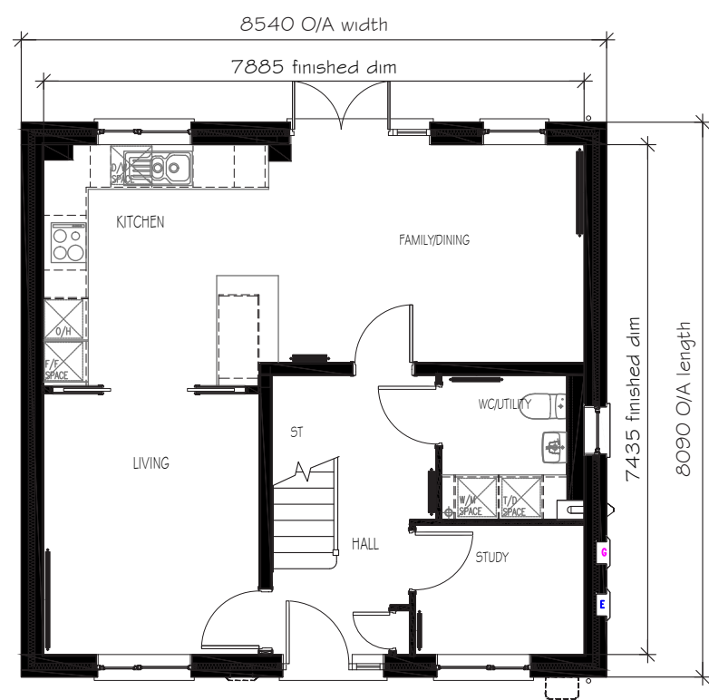
GROUND FLOOR PLAN - AS EMB51 (5B7P)
