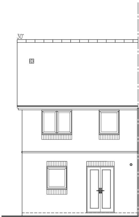
REAR ELEVATION END/SEMI DETACHED EMA32 (3B5P)
