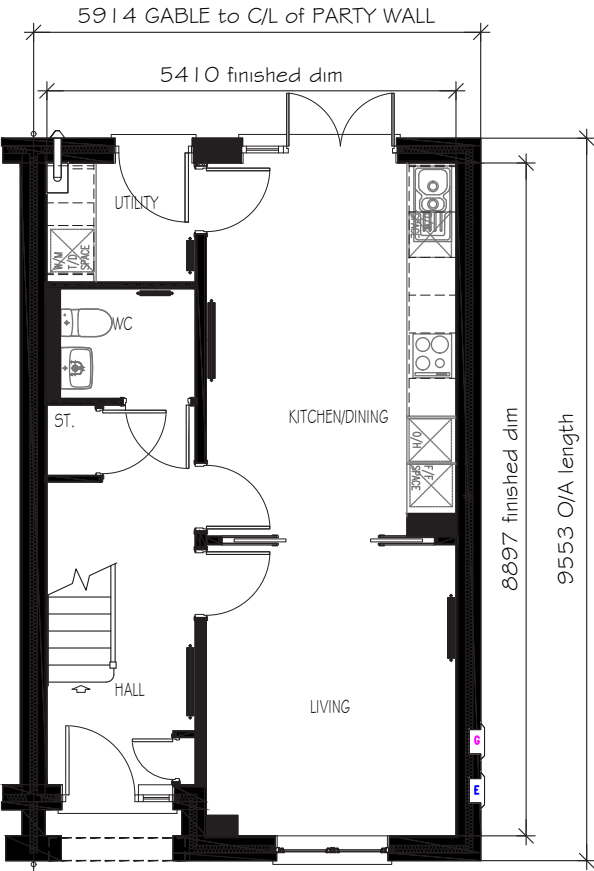
GROUND FLOOR PLAN (END/SEMI) EMA35 (3B5P)
