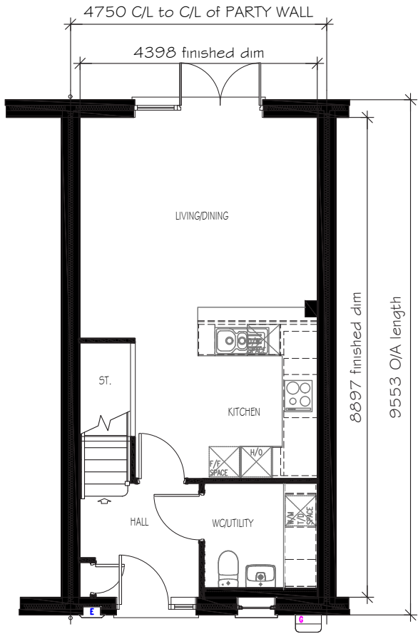
GROUND FLOOR PLAN (MID) EMB31 (3B5P)
