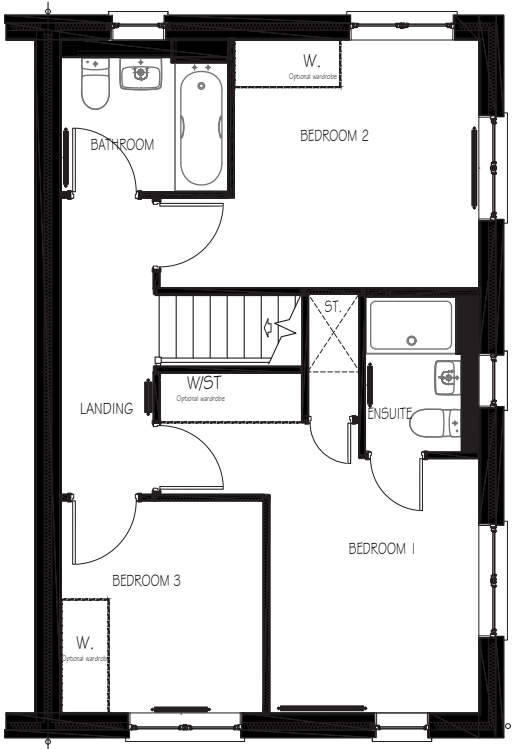
FIRST FLOOR PLAN (END/SEMI) EMT31 (3B5P)
