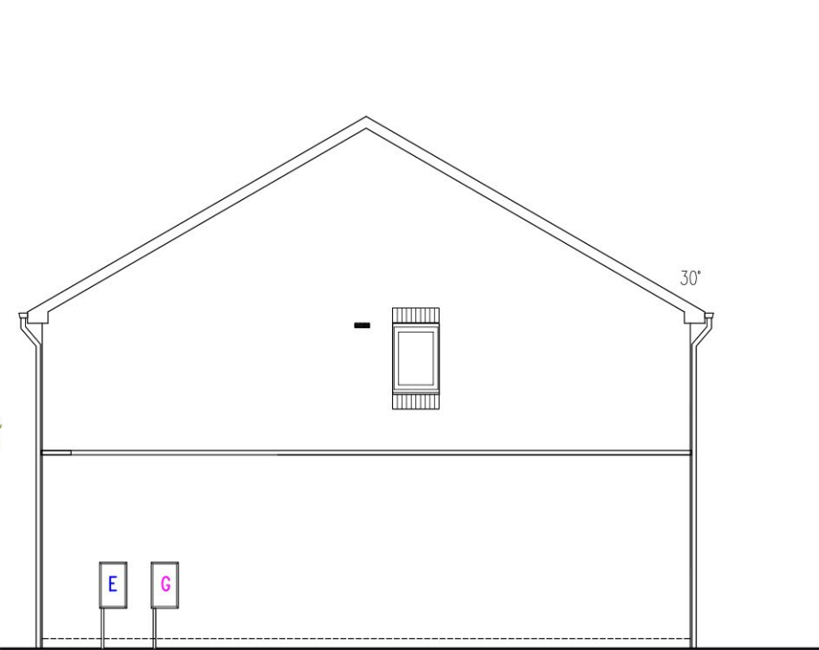
SIDE (RIGHT) ELEVATION END/SEMI DETACHED EMA35 (3B5P)
