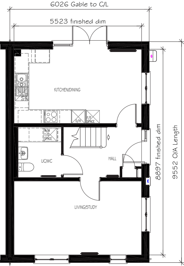
GROUND FLOOR PLAN (END/SEMI) EMT31 (3B5P)
