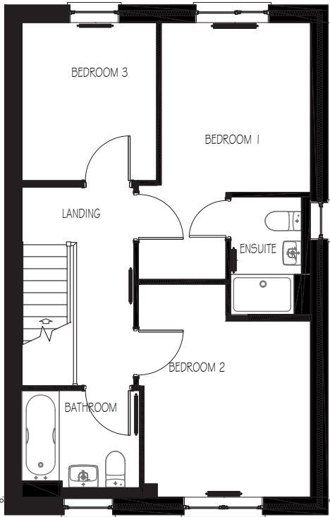
FIRST FLOOR PLAN (DETACHED) EMA35 (3B5P)
