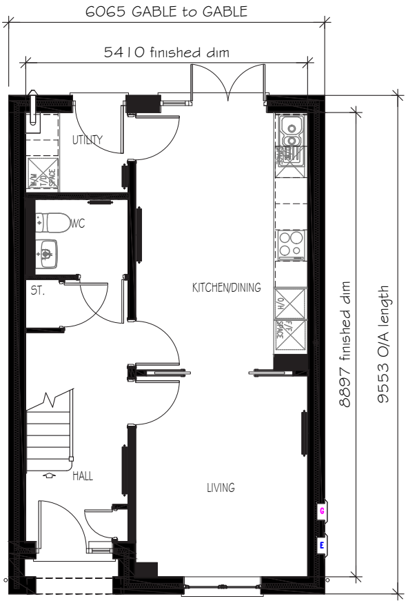
GROUND FLOOR PLAN (DETACHED) EMA35 (3B5P)
