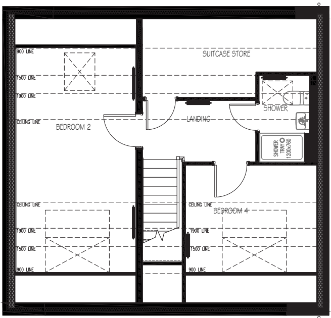
SECOND FLOOR PLAN - AS EMB51 (5B7P)
