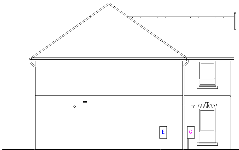
SIDE (RIGHT) ELEVATION DETACHED EMG42 (4B7P)
