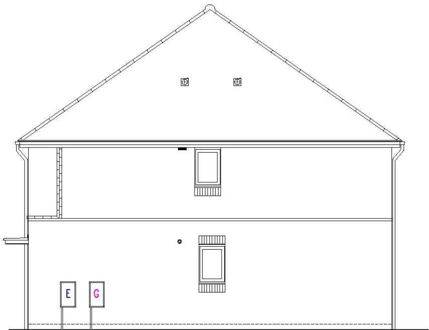
SIDE (RIGHT) ELEVATION END/SEMI DETACHED EMA41 (4B6P)
