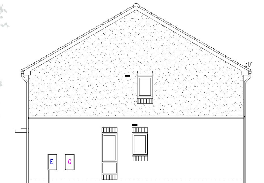
SIDE ELEVATION END/SEMI DETACHED (RIGHT) EMA32 (3B5P)
