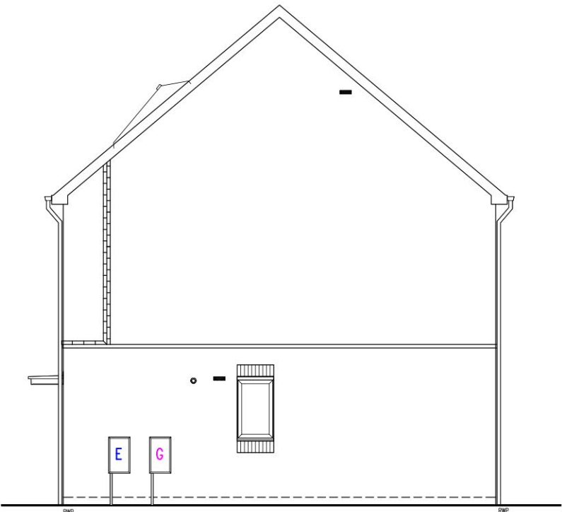
SIDE (RIGHT) ELEVATION - AS DETACHED EMB51 (5B7P)
