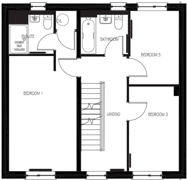
FIRST FLOOR PLAN - AS EMB51 (5B7P)
