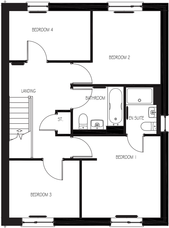
FIRST FLOOR PLAN (DETACHED) - AS EMA43 (4B5P)
