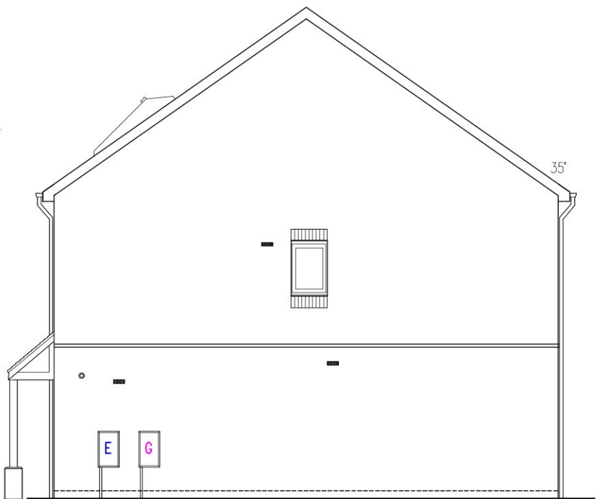
SIDE ELEVATION END/SEMI DETACHED (RIGHT) EMB31 (3B5P)
