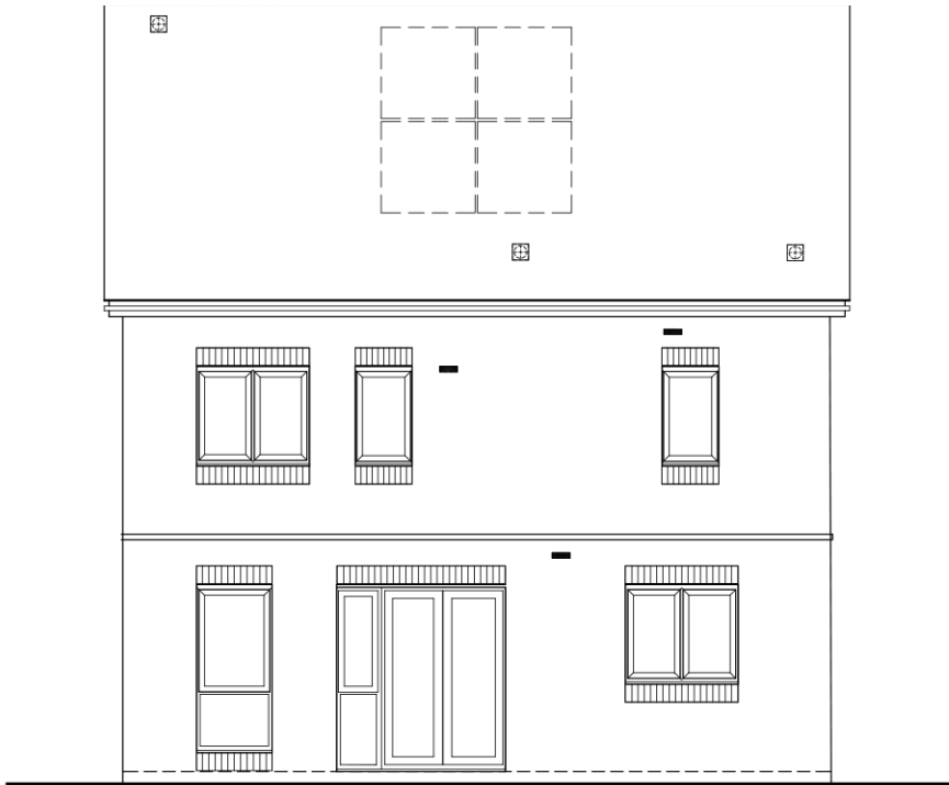
REAR ELEVATION - AS DETACHED EMB51 (5B7P)
