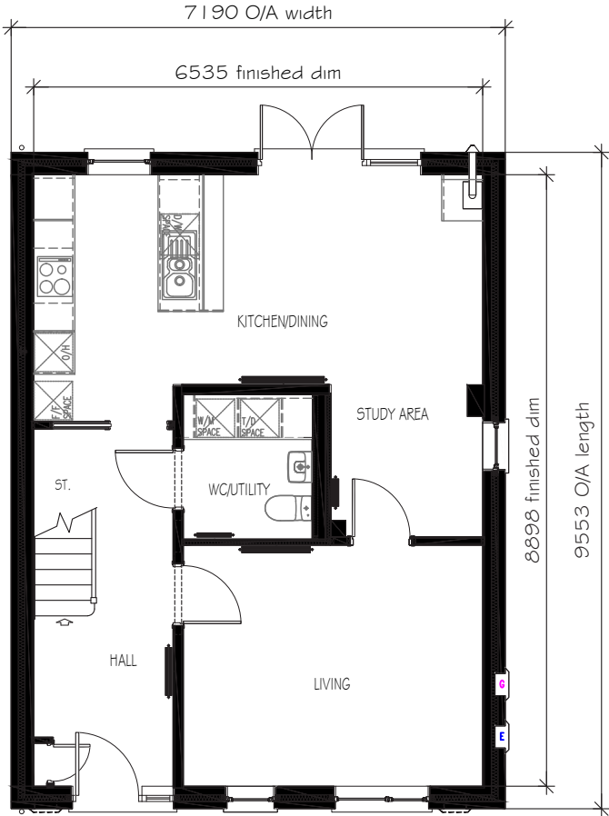
GROUND FLOOR PLAN (DETACHED) - AS EMA43 (4B5P)
