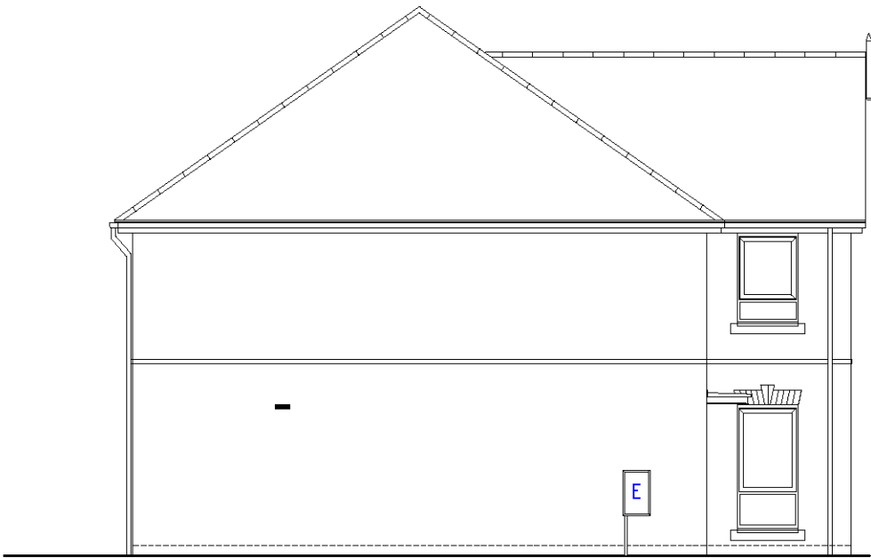
SIDE (LEFT) ELEVATION - AS DETACHED
