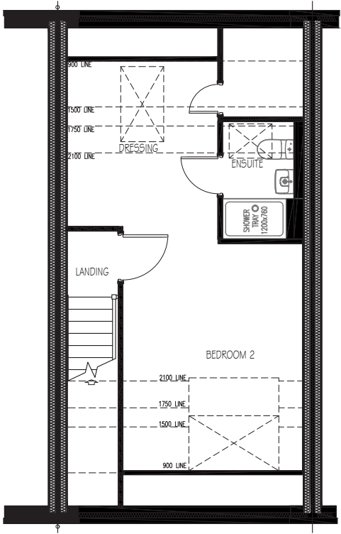
SECOND FLOOR PLAN (MID) EMB31 (3B5P)
