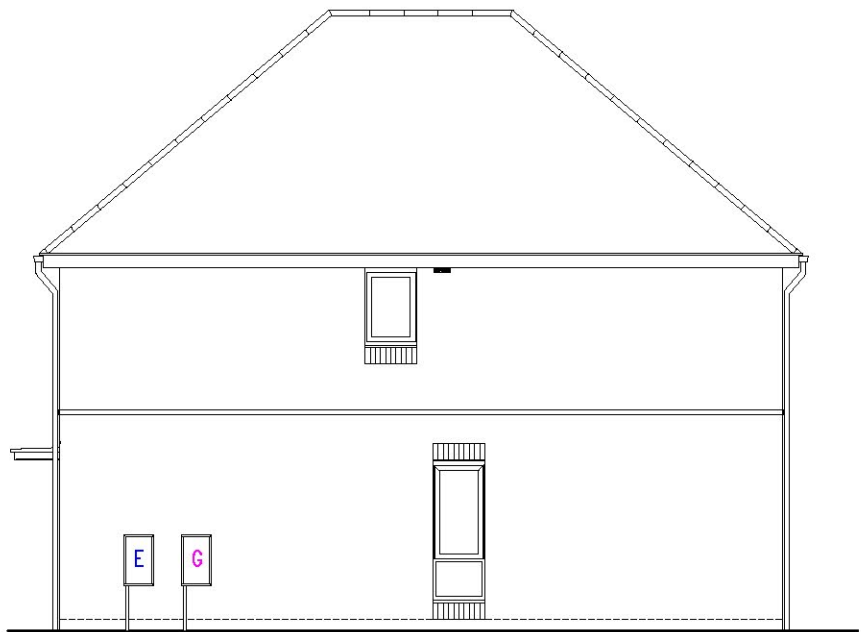
SIDE (RIGHT) ELEVATION - AS DETACHED EMA43 (4B5P)
