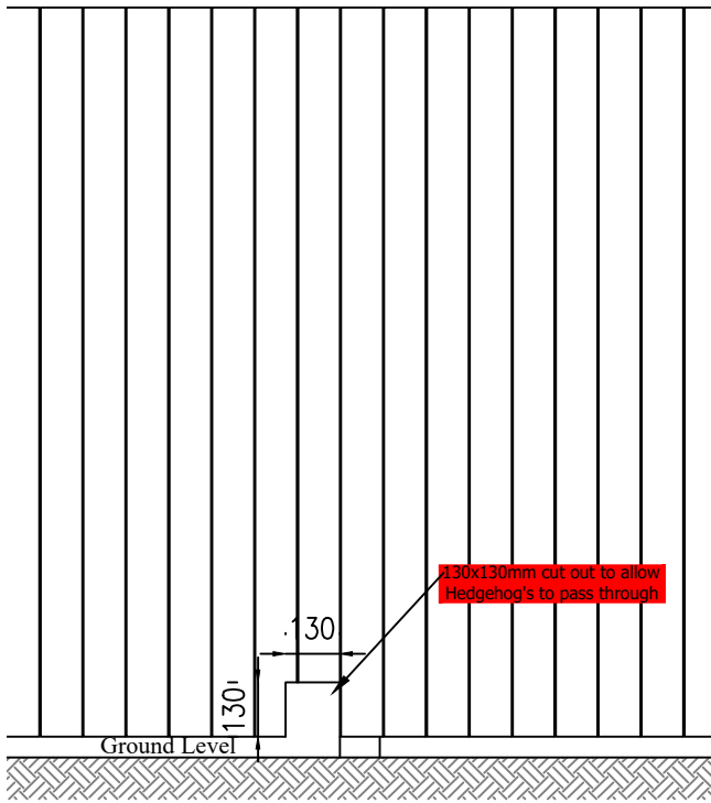
Front Elevation
