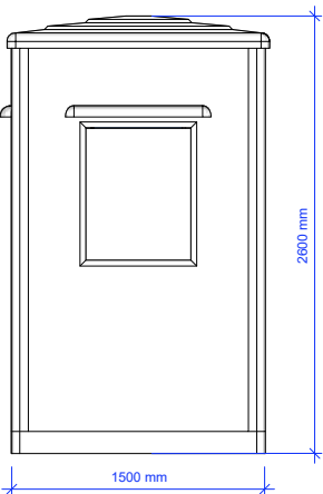
SIDE ELEVATION
