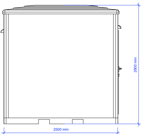
REAR ELEVATION
