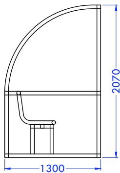
ELEVATION/SECTION
