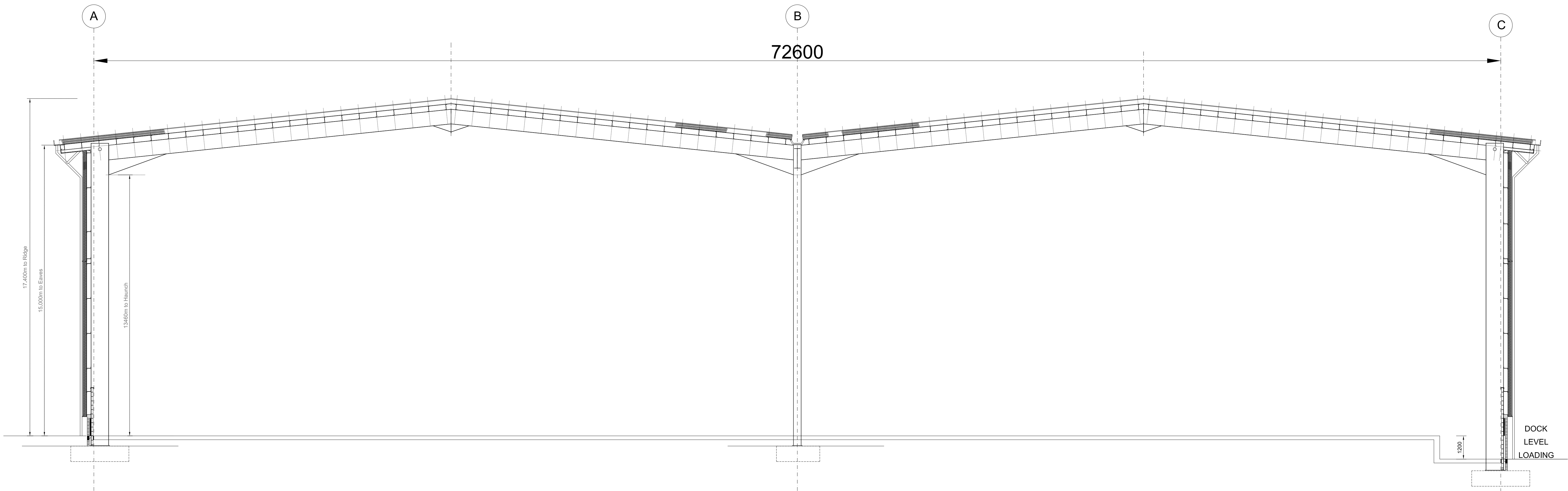
PROPOSED BUILDING OVERALL CROSS SECTION @ scale 1:100
