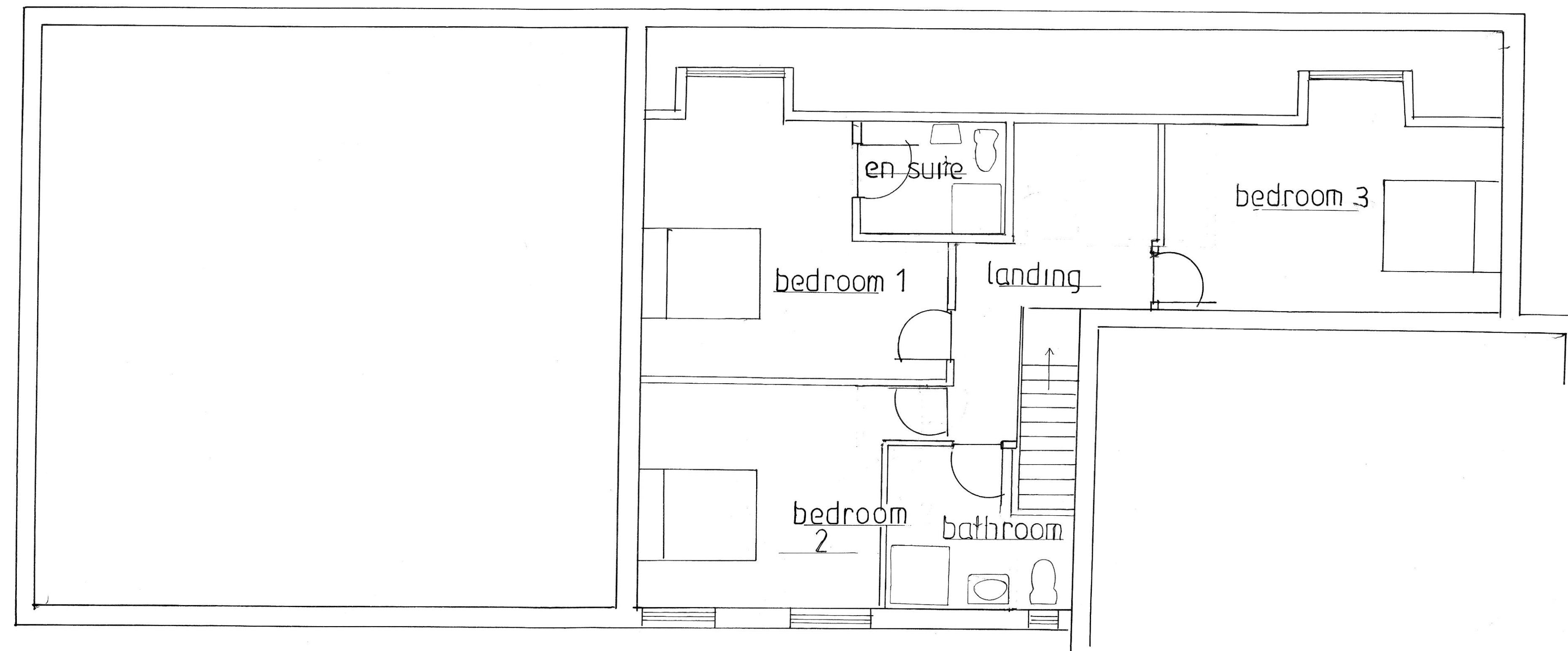
EXISTING FIRST FLOOR NO. 7 SCALE 1:50
