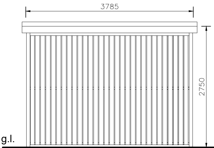
KEG STORE: WESTERN ELEVATION
