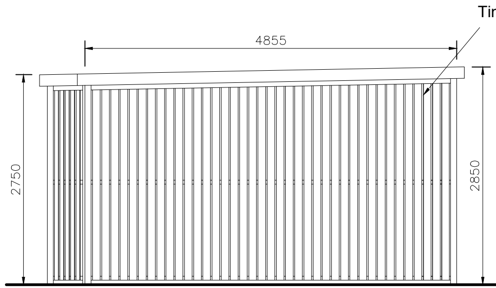
KEG STORE: SOUTHERN ELEVATION
