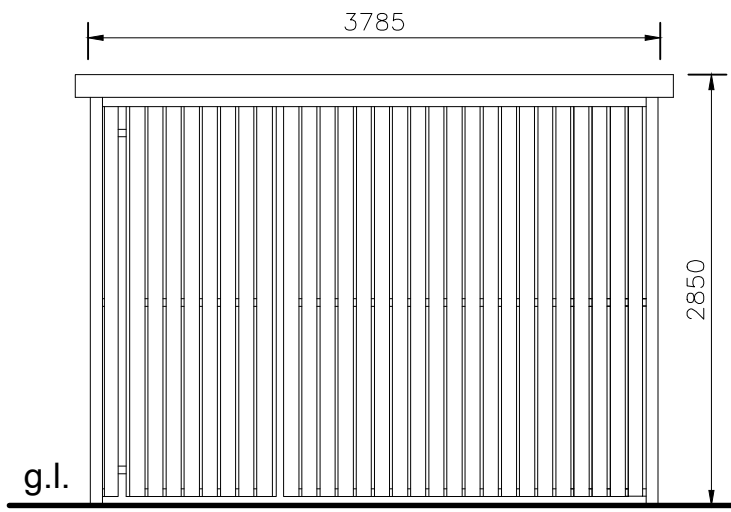
KEG STORE: EASTERN ELEVATION
