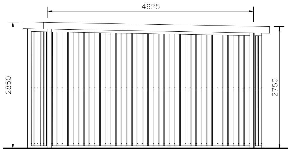
KEG STORE: NORTHERN ELEVATION
