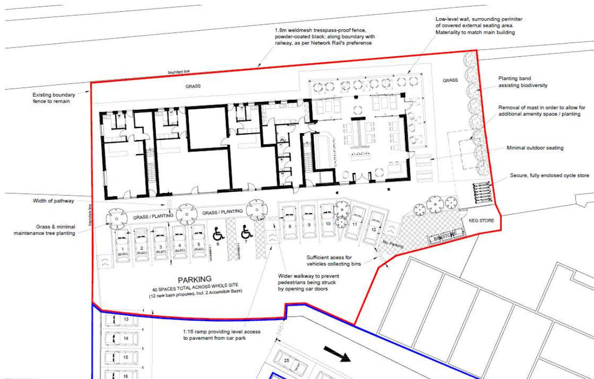
Figure 11 – Excerpt from 01823-SK-03 showing the proposed site plan
