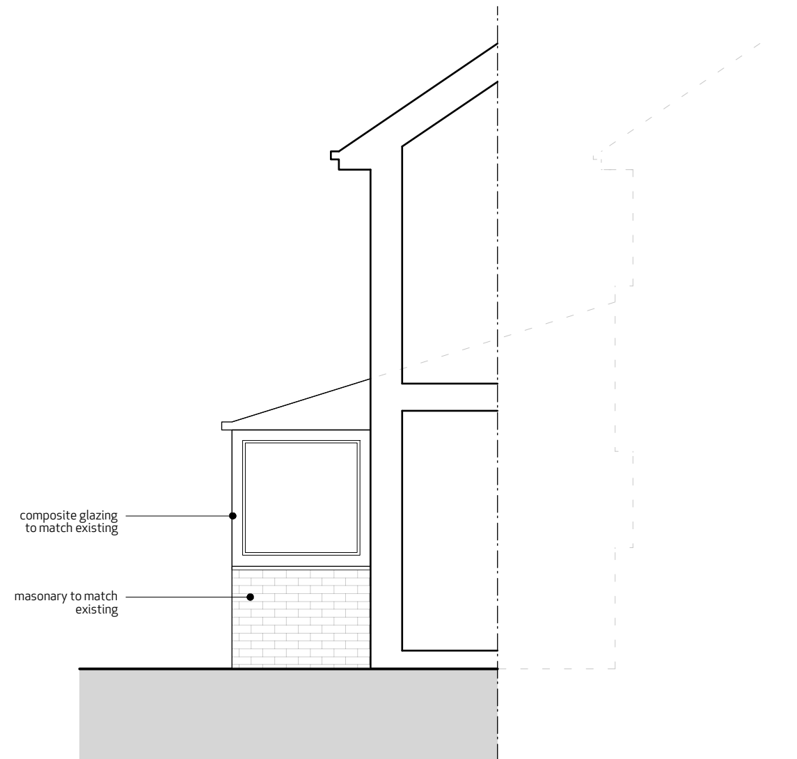
side elevation
