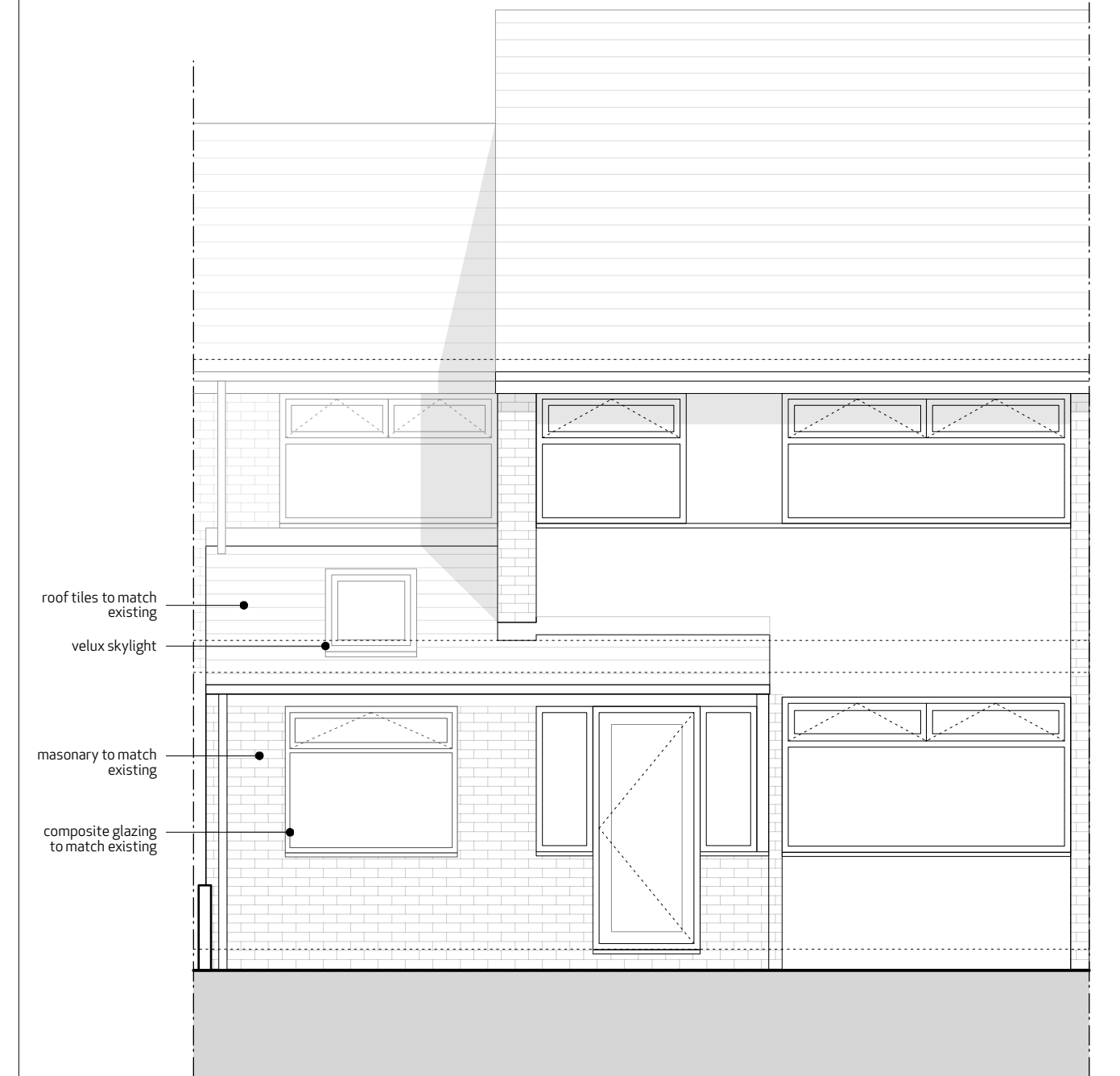
front elevation
