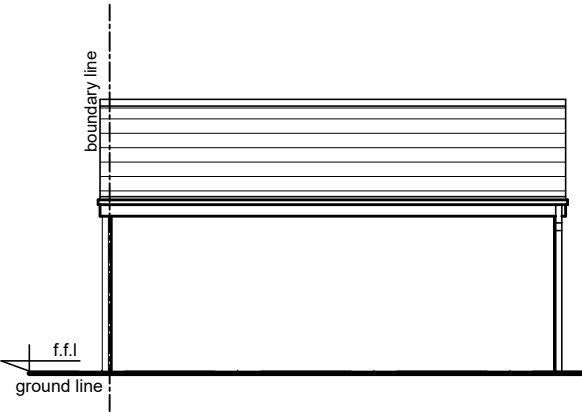
LEFT ELEVATION
