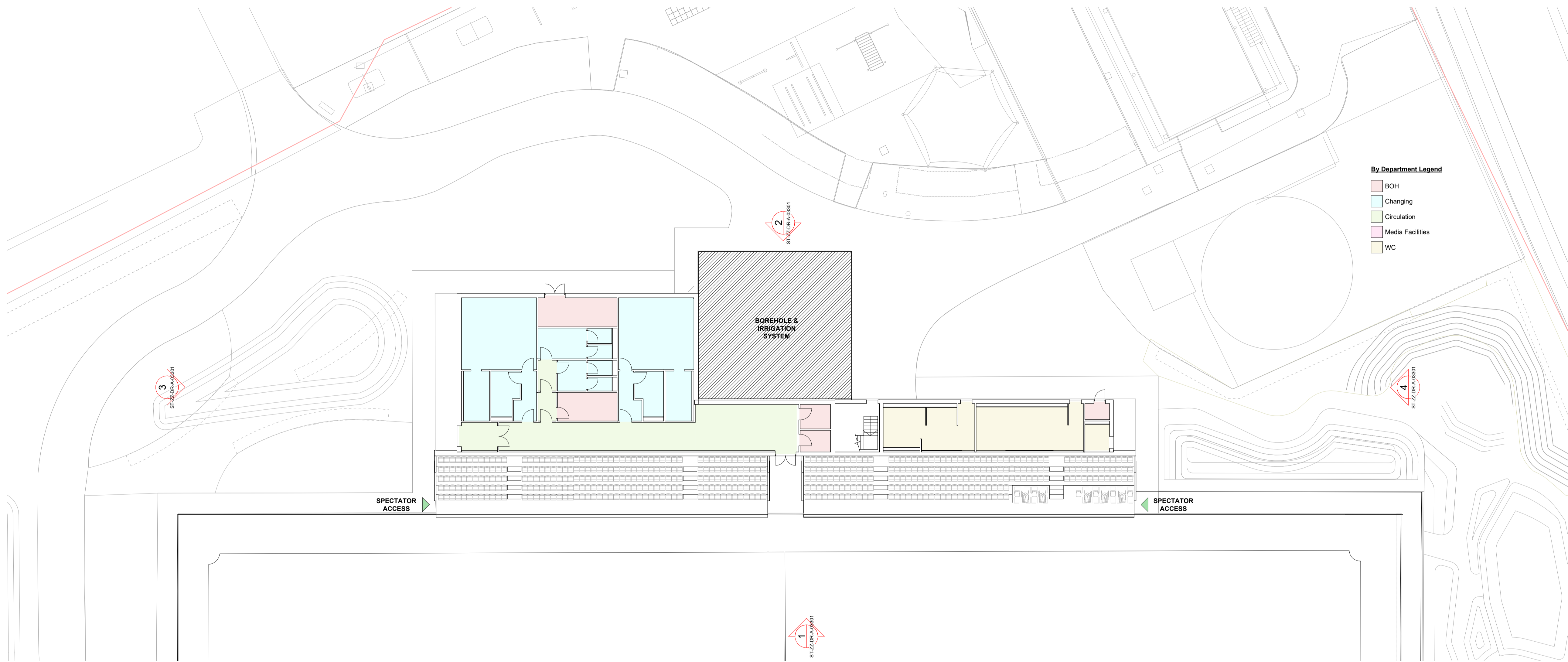
1 PLAN 00-PLANNING PROPOSED GROUND FLOOR PLAN 1 : 200
