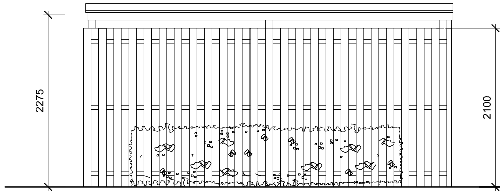
side elevation (facing fence)
