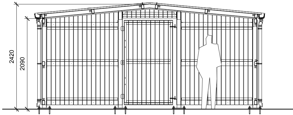
front elevation
