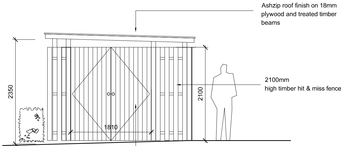
Front elevation (facing Paradise Lane)
