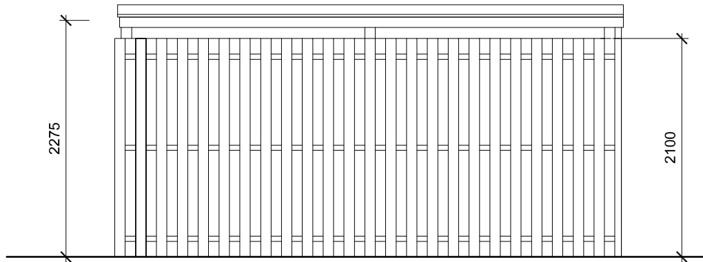
side elevation (facing Block C)
