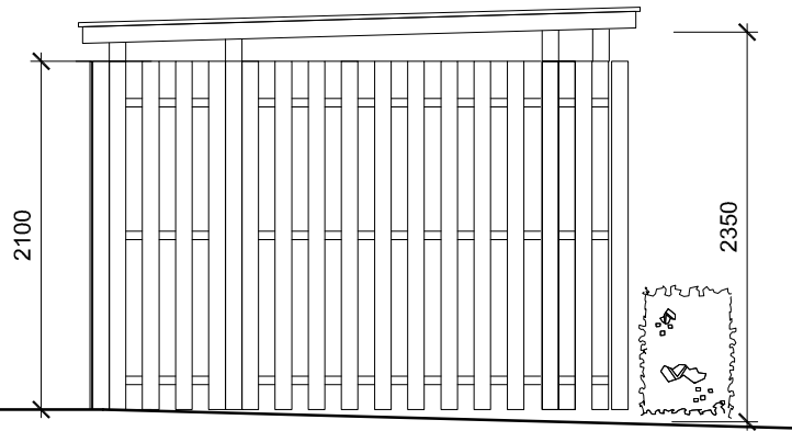
Front elevation (facing Paradise Lane)
